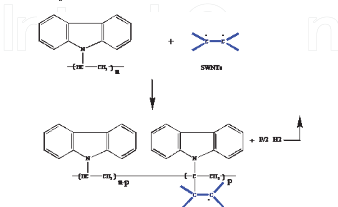
Fig. 7. Covalent bonding of OVK on the SWNTs side wall.
