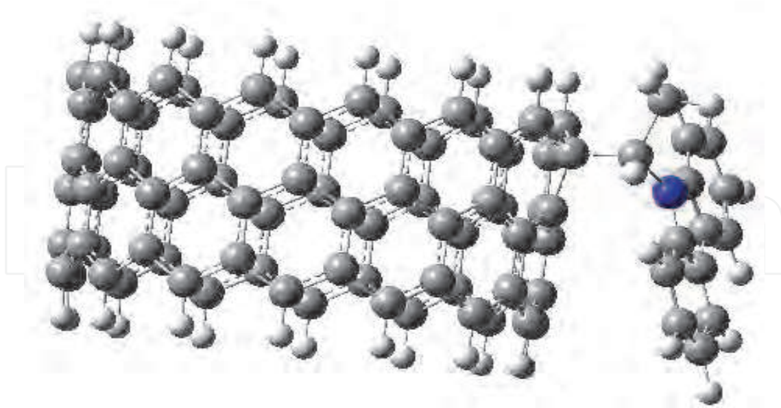
Fig. 14. OVK/SWNTs modelling structure.
