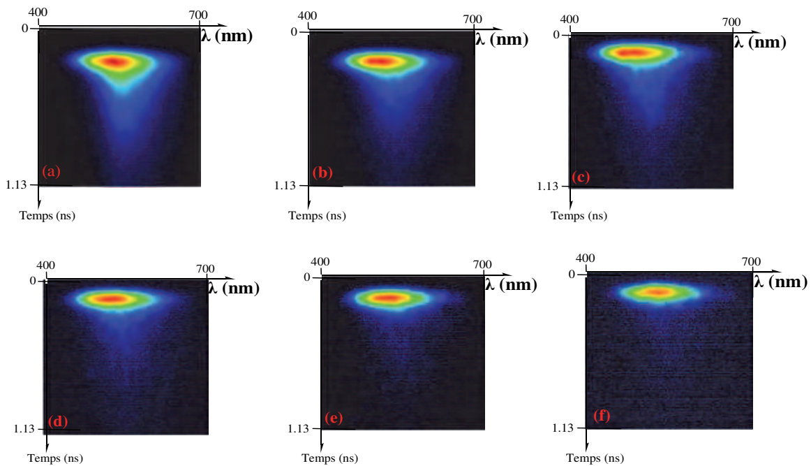
Fig. 20. Transient photoluminescence contour maps in false color of standard PVK-H3T (a) and those of PVK-3HT/SWNTs composites for different mass concentrations x of SWNT. (a) Standard PVK-3HT, (b) x=1.87\% , (c) x=7.5\% , (d) x=15\% , (e) x=30\% , (f) x=60\% .
