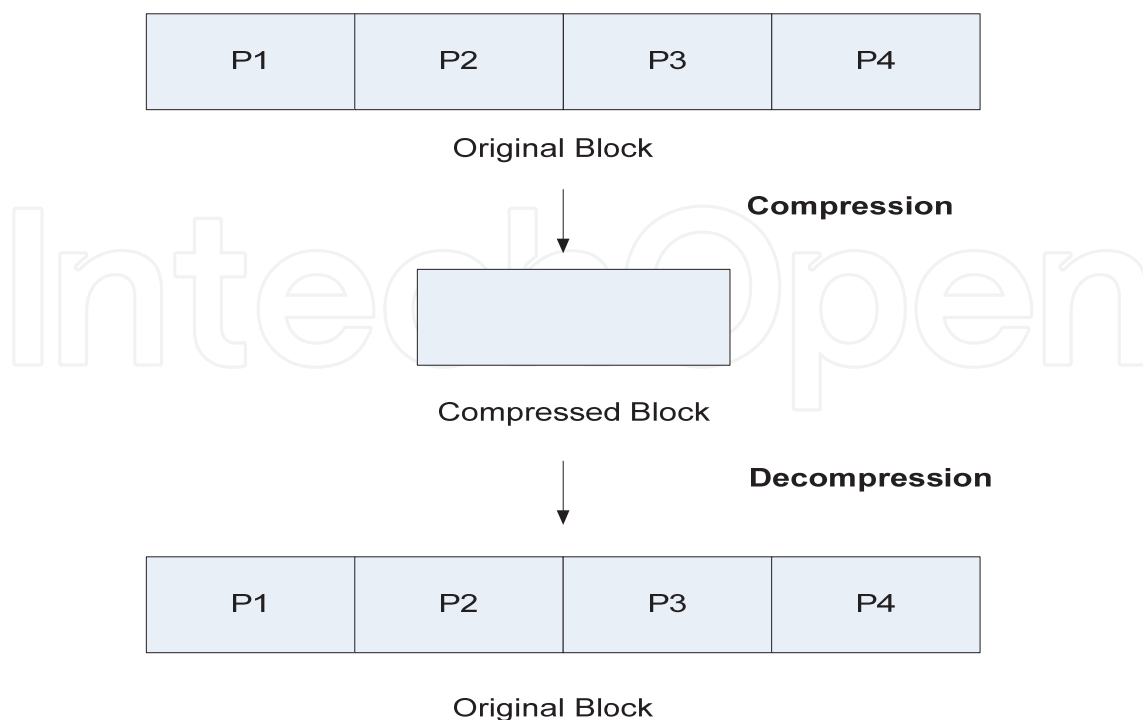
Fig. 12. Block compression.
