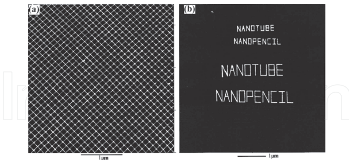
Fig. 14. AFM image of 2 nm tall, 10 nm wide, and 100 nm spaced silicon-oxide (light) lines fabricated by a nanotube tip using anodic oxidation method (Dai & Franklin, 1998).
