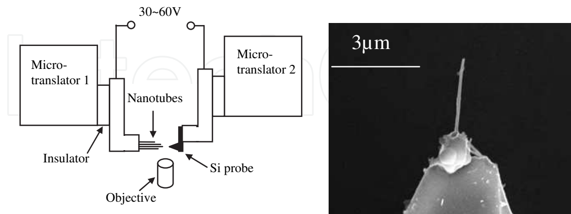
Fig. 2. Schematic illustration of welding process and CNT probe fabricated (Fang et al., 2007)
