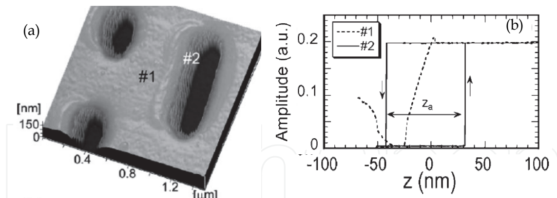
Fig. 10. The CNT probe image of a DVD surface (a), and the force curve measurement performed near the pit edge and on a plane surface (b) (Akita et al., 2000a).
