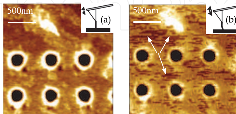
Fig. 13. Nanoholes images captured by CNT probe with 18nm (a) and 40nm (b) scan amplitudes (Fang et al., 2009).
