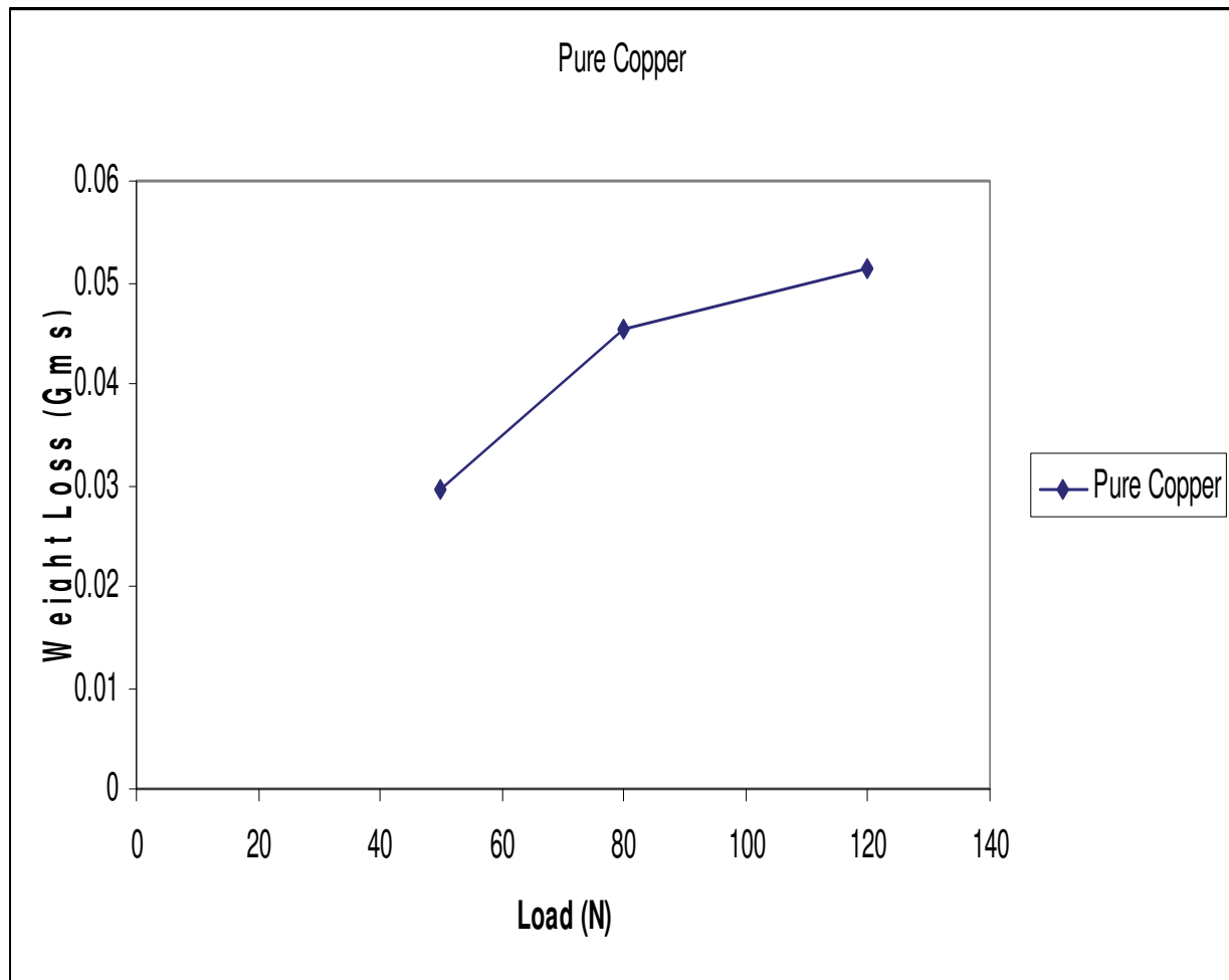
Fig. 15. Load Vs Weight loss
