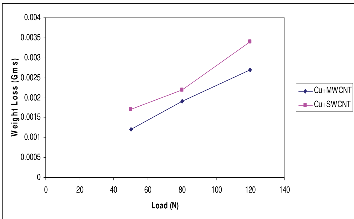
Fig. 14. Load Vs Weight loss
