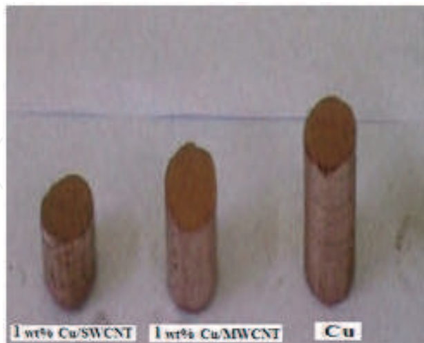
Fig. 4. Powder Compacted (Pre-sintered) Wear Test Specimens
