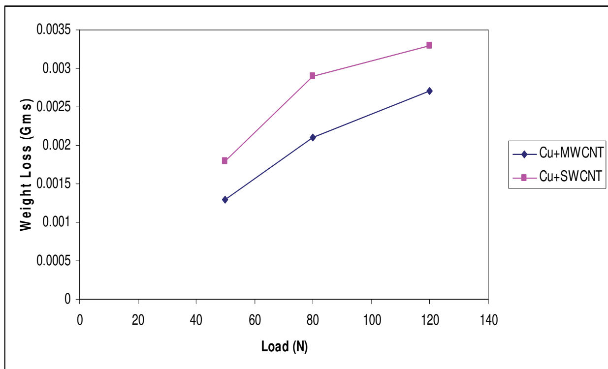
Fig. 13. Load Vs Weight loss
