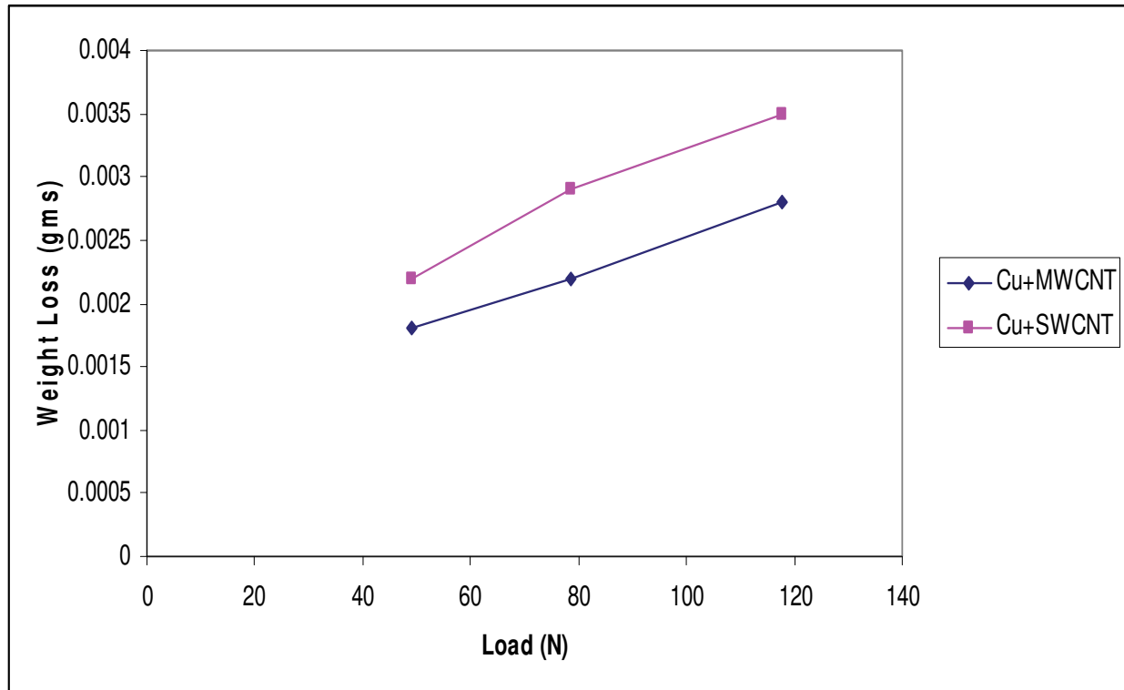
Fig. 12. Load Vs Weight loss
