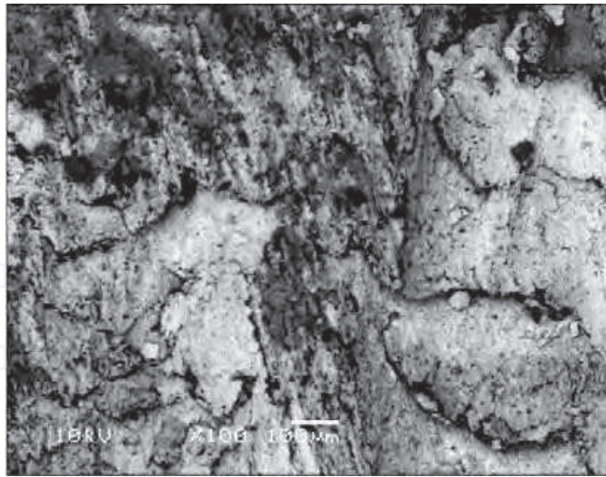
Fig. 5. SEM Image of Wear Tested Pure Cu sample
