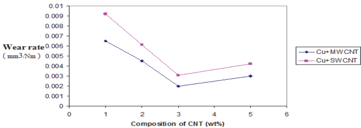
Fig. 11. CNT Composition Vs Wear rate
