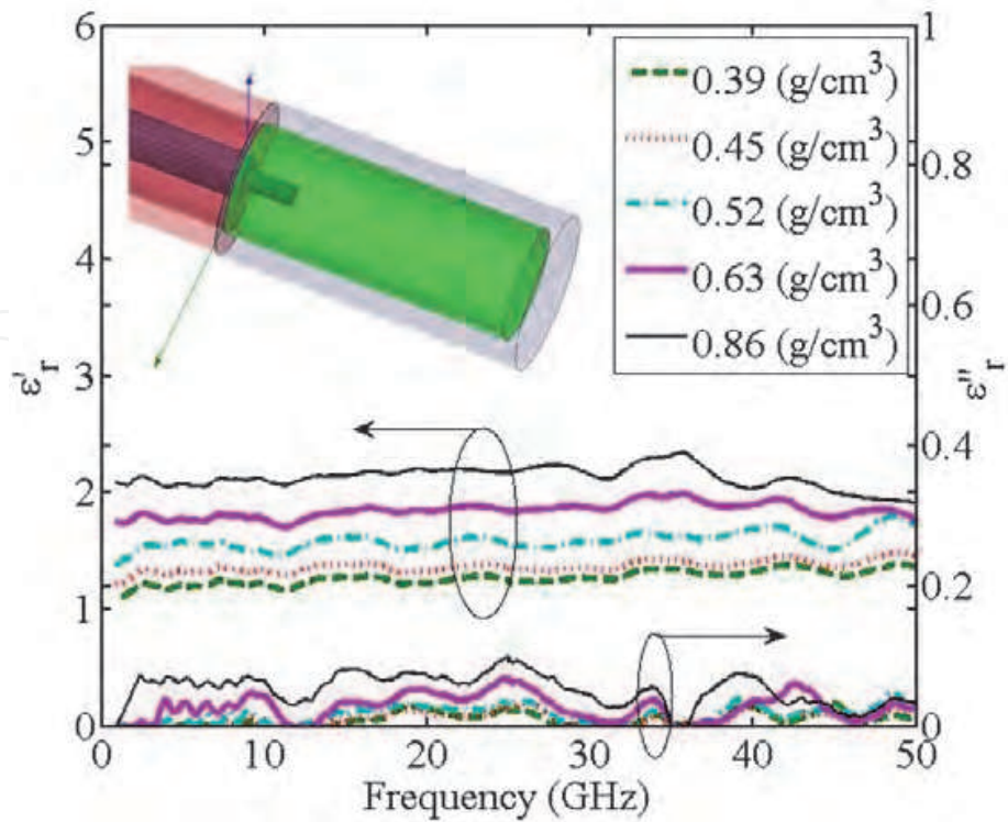
Fig. 3. Variation of extracted effective permittivity of pure pulverized \text{SiO}_2 versus frequency using the test setup as shown in Fig. 1.
