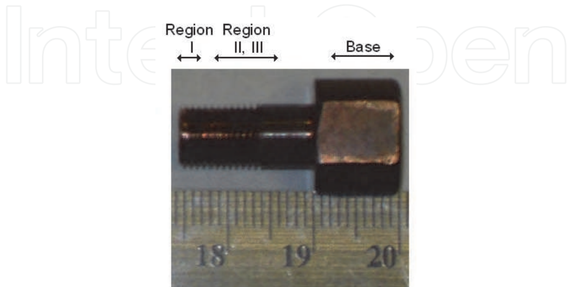
Fig. 2. Actual picture of the fabricated testing structure. Regions I, II, and III are the same as those shown in the schematic of Fig. 1. Dimensions of design parameters shown in Fig. 1 are: a = 1.2 mm, b = 0.52 mm, a_1 = 1.26 mm, b_1 = 0.254 mm, L_1 = 1.1 mm, L_2 = 5.3 mm.
