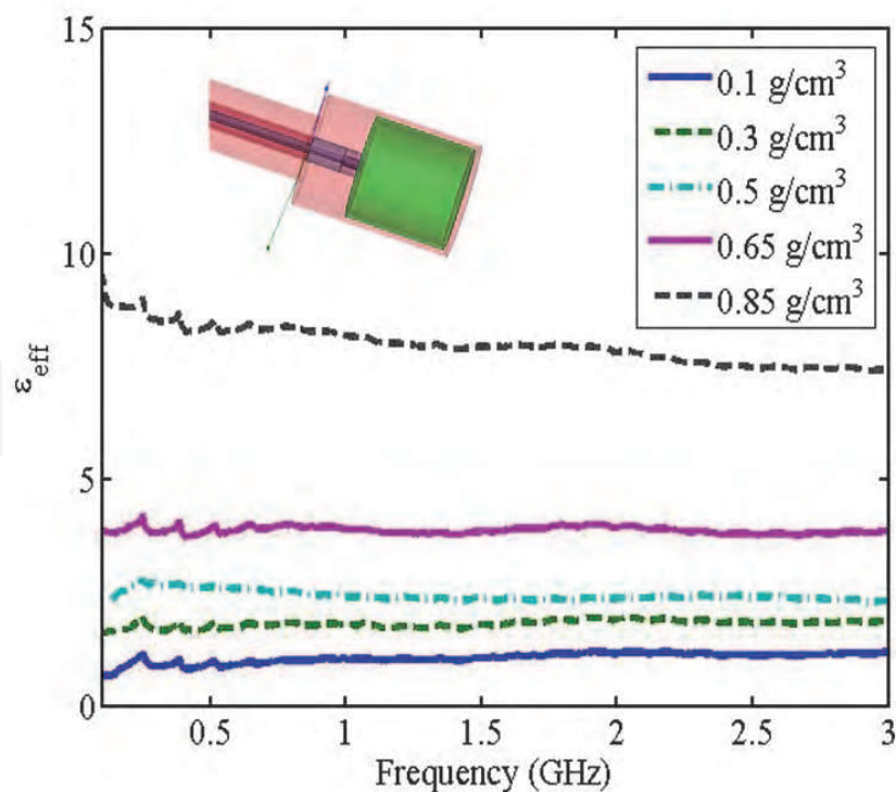
Fig. 17. Variation of extracted real part of the effective permittivity of carbon nanotubes mixed with alumina versus frequency using the test setup as shown in the inset.
