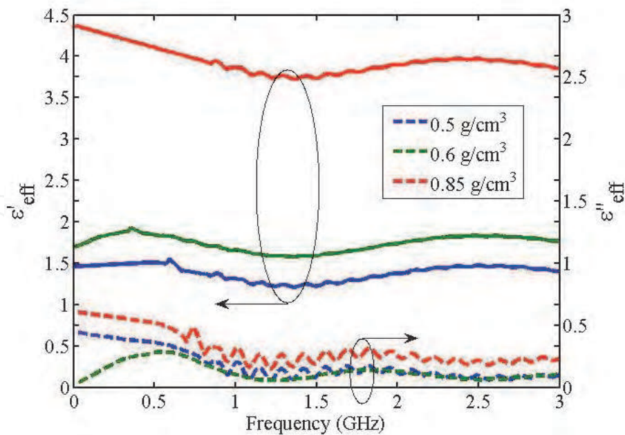
Fig. 14. Extraction of the complex effective permittivity ( \epsilon_{eff} = \epsilon'_{eff} - j\epsilon''_{eff} ) considering the 75% weight mixture of Alumina-copper for different densities functions of the frequency using the test setup shown in Fig. 1.
