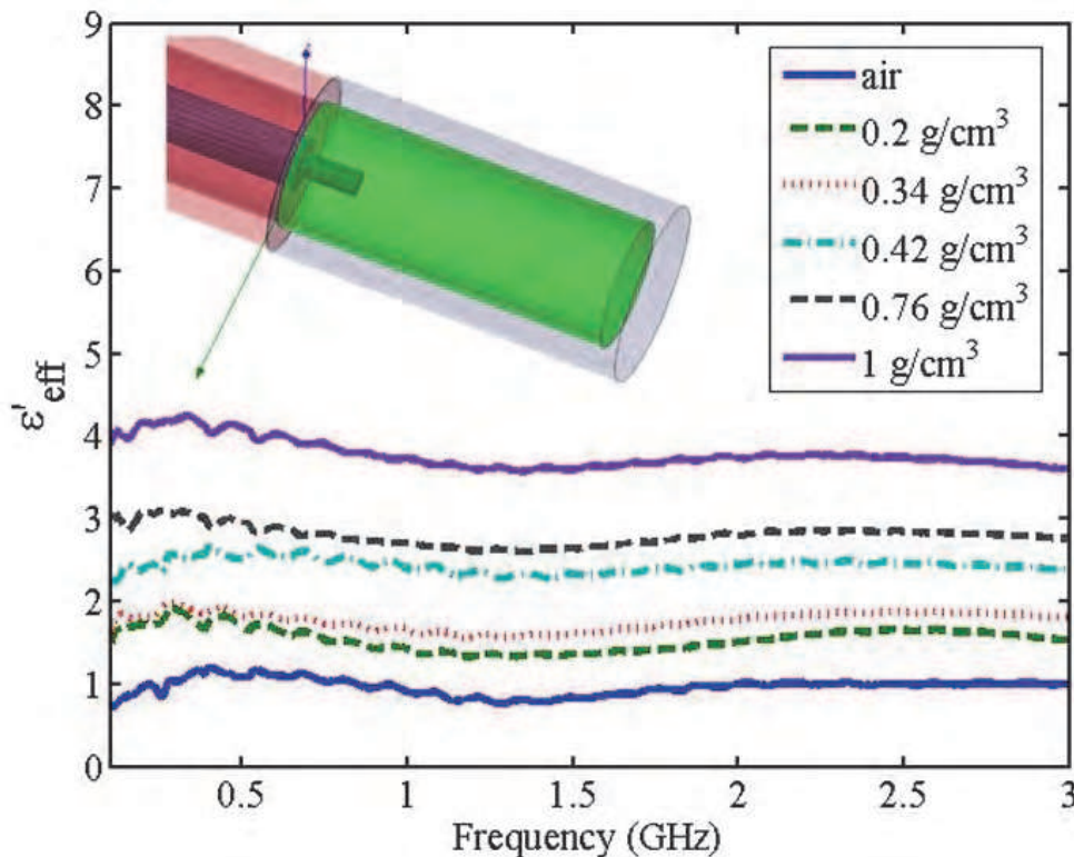
Fig. 5. Variation of extracted effective dielectric constant of pure \text{Al}_2\text{O}_3 powder versus frequency at different densities using the test setup shown in Fig. 1.
