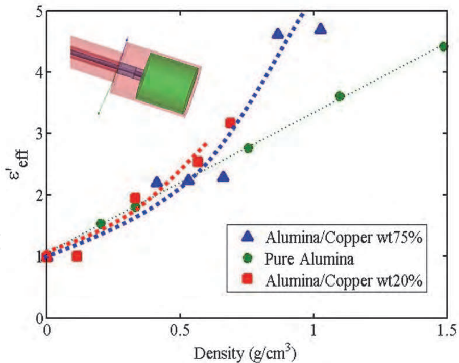
Fig. 15. Variation of the effective permittivity of the composite material function of the density realized at 60MHz and compared to pure alumina powder.
