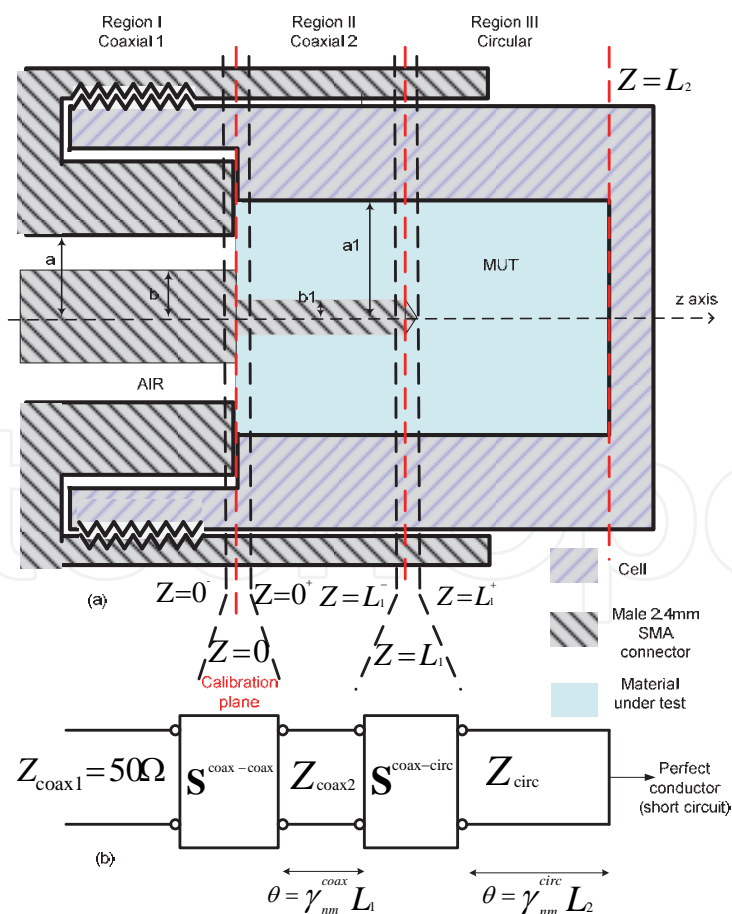
Fig. 1. (a) Schematic of the test structure. (b) Generalized scattering matrices building blocks.
