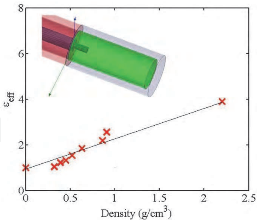
Fig. 4. Variation of extracted effective permittivity of pure \text{SiO}_2 versus density realized at frequency of 3GHz. The last point is the common accepted value for \text{SiO}_2 , \epsilon_{\text{eff}} = 3.9 for a density of 2.2 \text{ g/cm}^3 .
