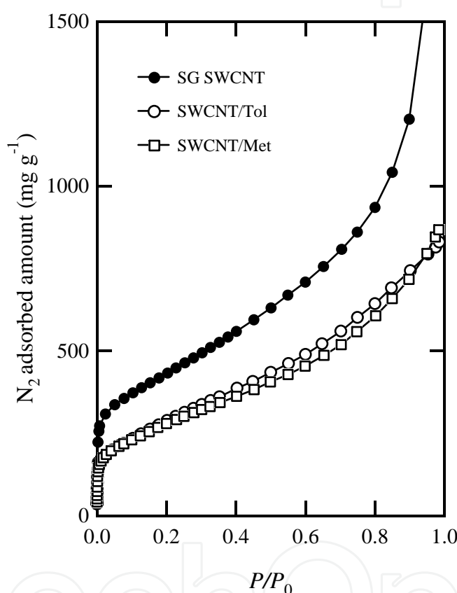
Fig. 16. \text{N}_2 adsorption isotherms of SG SWCNT (●), SWCNT/Tol (○), and SWCNT/Met (□) at 77 K.
