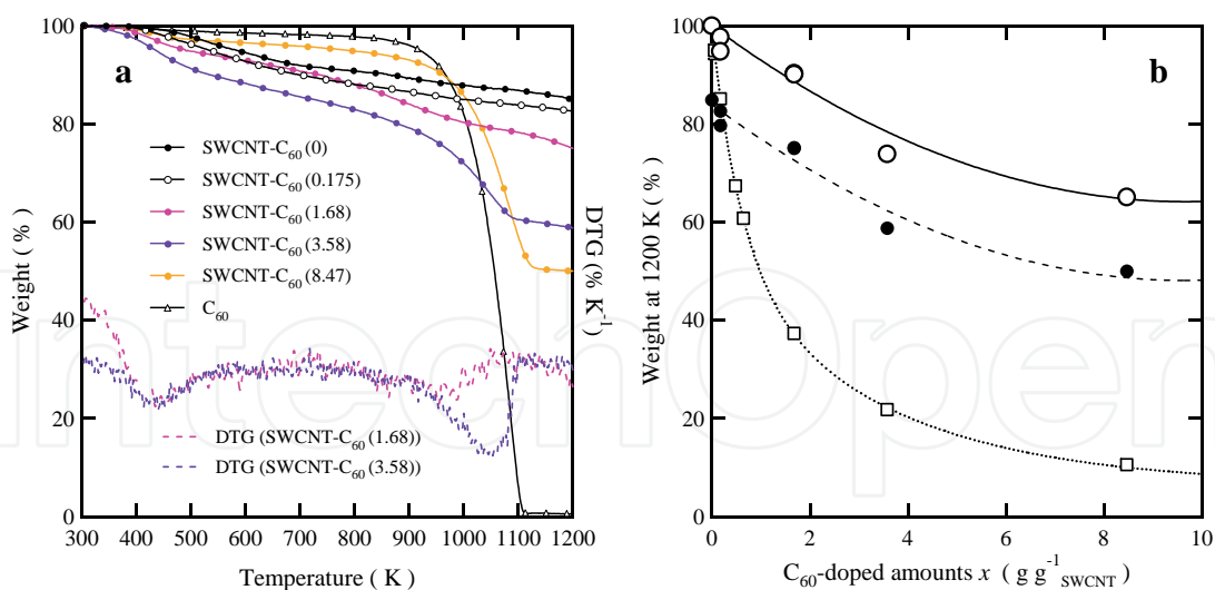
Fig. 10. TGA of SWCNT- C_{60}(x) samples and C_{60} . (a) TG and typical DTG ( x : 1.68 and 3.58) curves of SWCNT- C_{60}(x) and C_{60} . (b) Closed circles (●) indicate the weight percents ( TG_{1200\text{K}} ) of the sample weight at 1200 K against the initial sample weight with C_{60} -doped amount. Open circles (○) indicate the weight change at 1200 K of SWCNT- C_{60} , after correction of the weight decrease of SWCNT itself. Open squares (□) correspond to the theoretical weight decrease in percent of SWCNT- C_{60}(x) under the assumption that doped- C_{60} is completely sublimated.
