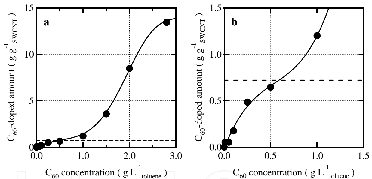
Fig. 3. C_{60} -doped amount on SWCNT bundles against the concentration of C_{60} -toluene solutions. (a) Relationship between the C_{60} -doped amount on 1 g of SWCNT samples ( g g^{-1}_{SWCNT} ) and the concentration of C_{60} -dissolved toluene. (b) Magnified view of Fig. 3a. The broken lines indicate the expected C_{60} -doped amount corresponding to perfect filling of the interstitial nanospaces with C_{60} in the model structure of C_{60} -pillared SWCNT bundles with hexagonal symmetry.
