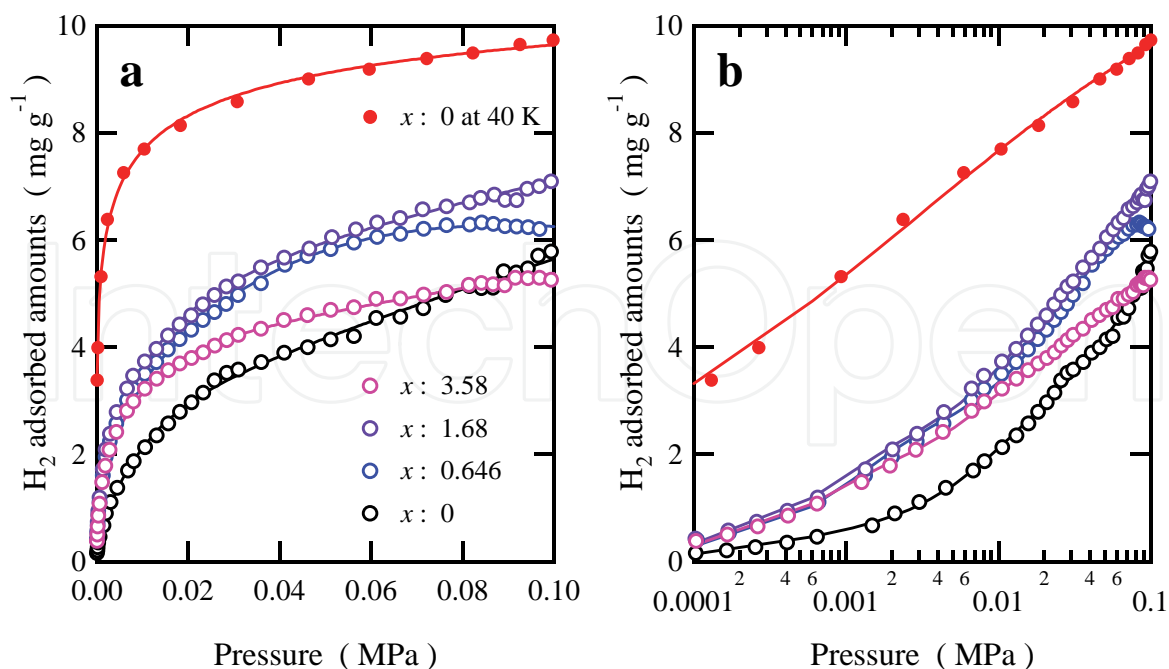
Fig. 13. H_2 adsorption isotherms of SWCNT- C_{60}(x) at 77 K. For comparison, the isotherm of SWCNT- C_{60}(0) measured at 40 K is also shown. The abscissas of a and b are expressed by the H_2 pressure and the logarithm of the H_2 pressure, respectively.
