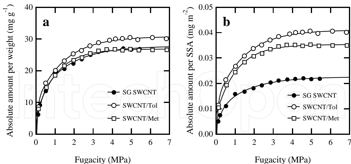
Fig. 17. High pressure H_2 adsorption isotherms of SG SWCNT ( \bullet ), SWCNT/Tol ( \circ ), and SWCNT/Met ( \square ). The vertical axes of a and b are expressed by the absolute H_2 amounts per the weight and per the specific surface area of the samples, respectively.
