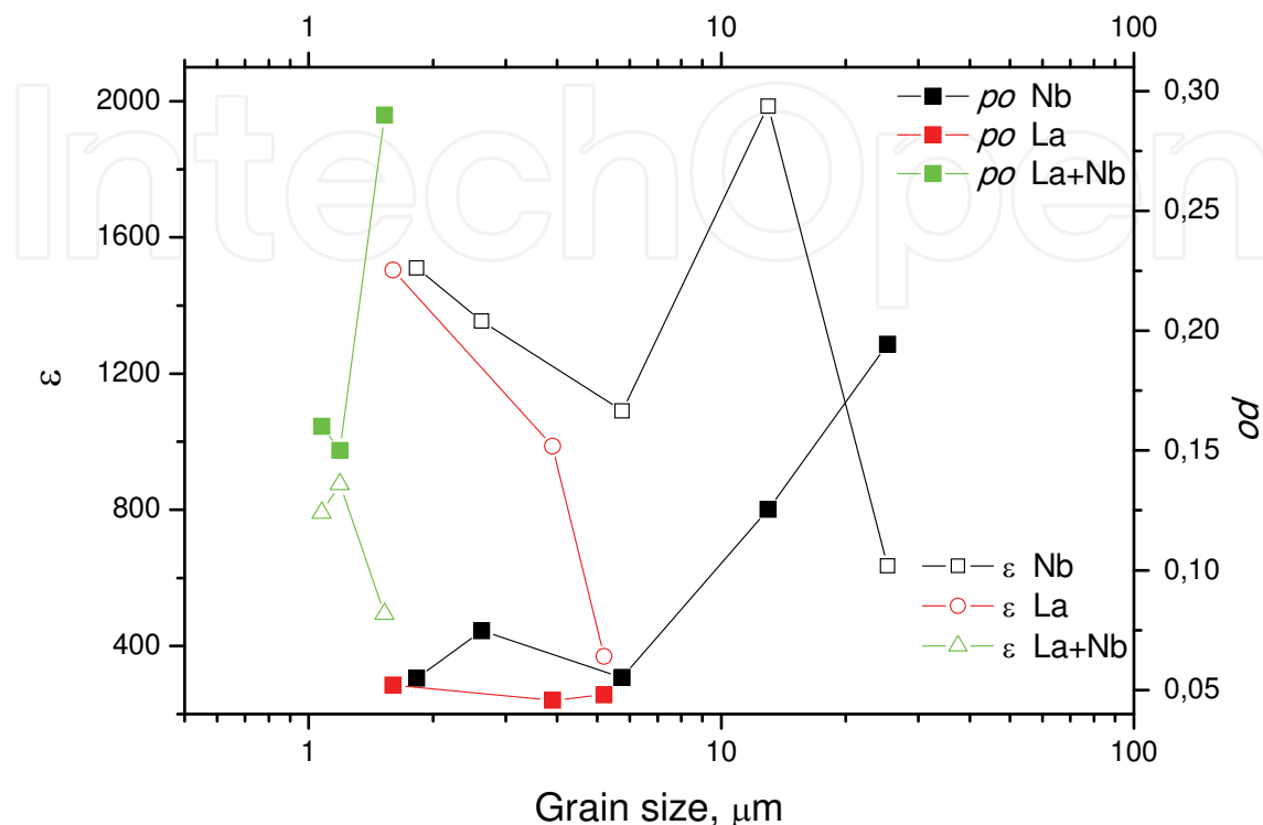
Fig. 16. Behavior at room temperature of dielectric constant ( · ) and porosity (po) as function of the grain size.
