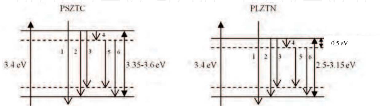
Fig. 12. Possible energetic process that will be happen in PZT ceramics. 3.4 eV is excitation energy (373 nm), 1-6 there are the possible recombination way (PL). We consider that occurred the way 1, 5 and 6 mainly.
