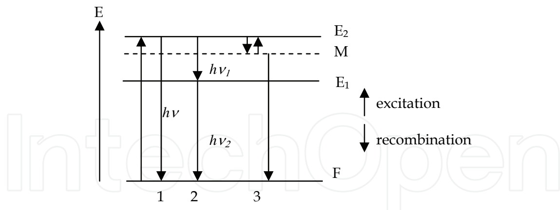
Fig. 1. Three possible luminescence types of an isolated atom:
