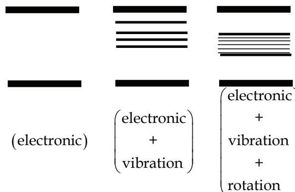
Fig. 2. Energy levels that appear in a molecule.
