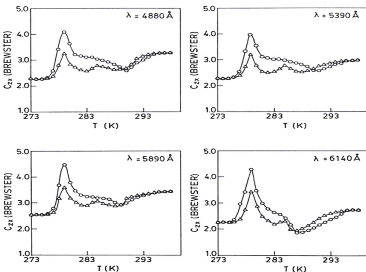
Fig. 21. Temperature dependence of photoelastic coefficient C_{zx} of the crystal (x-irradiated) LGO at different wave lengths in a cooling (○) and heating (△) cycle.
