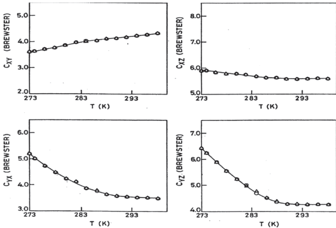
Fig. 15. Temperature dependence of the piezo-optic coefficients C_{xy} , C_{xz} , C_{yz} and C_{yx} of the crystals LGO in a cooling ( \circ ) and heating ( \Delta ) cycle.
