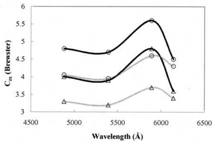
Fig. 22. The peak value of C_{zx} for the un-irradiated (black colour) and x-irradiated (ash colour) crystal LGO at different wave lengths in a cooling (0) and heating ( \Delta ) cycle.
