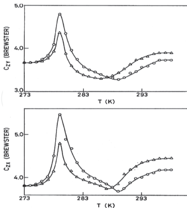
Fig. 16. Anomalous temperature dependence of the piezo-optic coefficients C_{zx} and C_{zy} of the crystals LGO in a cooling ( \circ ) and heating ( \Delta ) cycle.
