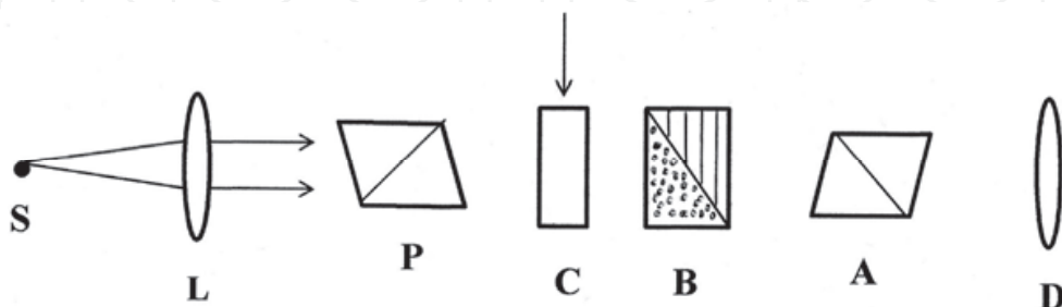
Fig. 2. A schematic diagram of the experimental setup for the measurement of photoelastic constants of the crystals at room temperature. Source of light (S), Lens (L), Polarizer (P), Crystals (C) under stress, Babinet Compensator (B), Analyzer (A) and Detector (D).
