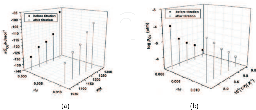
Fig. 12. Variation of (a) \Delta\bar{G}_{O_2} and (b) \log p_{O_2} with temperature and oxygen stoichiometry change for \text{Bi}_{0.90}\text{Ba}_{0.10}\text{Fe}_{0.90}\text{Ti}_{0.10}\text{O}_3
