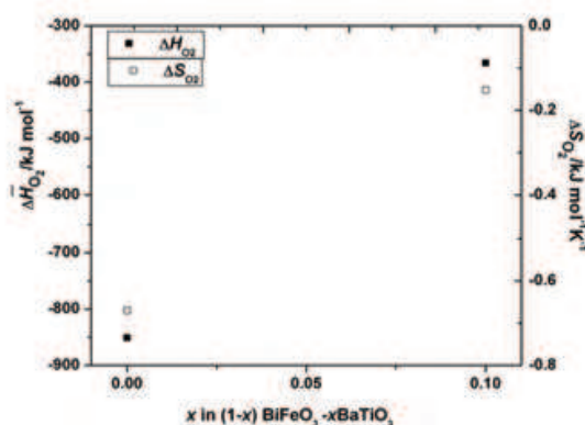
Fig. 11. \Delta\bar{H}_{O_2} and \Delta\bar{S}_{O_2} as a function of \text{BaTiO}_3 content ( x ) at temperatures lower than ferroelectric transition temperatures.
