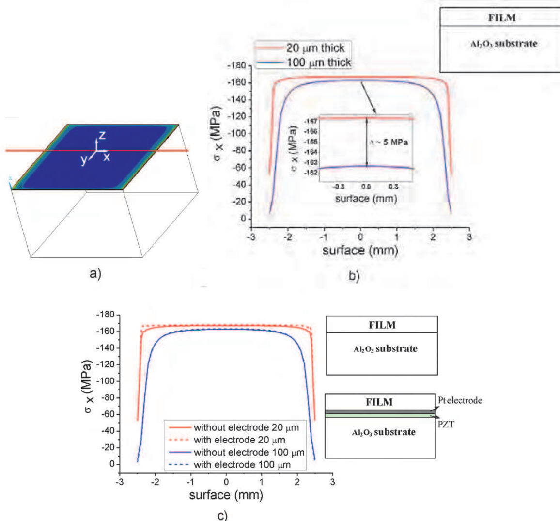
Fig. 4. (a) The model structure of the 0.65PMN–0.35PT film clamped on the thick alumina substrate and the \sigma_x distribution. The line shows the coordinates ( x , y = 0 , z = \text{top surface} ), where \sigma_x was calculated. (b) The \sigma_x vs. the position on the top surface of the 20- \mu\text{m} - and 100- \mu\text{m} -thick films. Inset: The enlarged central part of the graph. (c) The comparison of the \sigma_x shown in (b) with the updated calculation made for the structure including the Pt bottom electrode and the PZT barrier layer. Right: Schemes of the cross-section of the film-substrate structure (Reprinted with permission from [Uršič, H. et al., J. Appl. Phys. Vol. 109, No. 1.]. Copyright [2011], American Institute of Physics).
