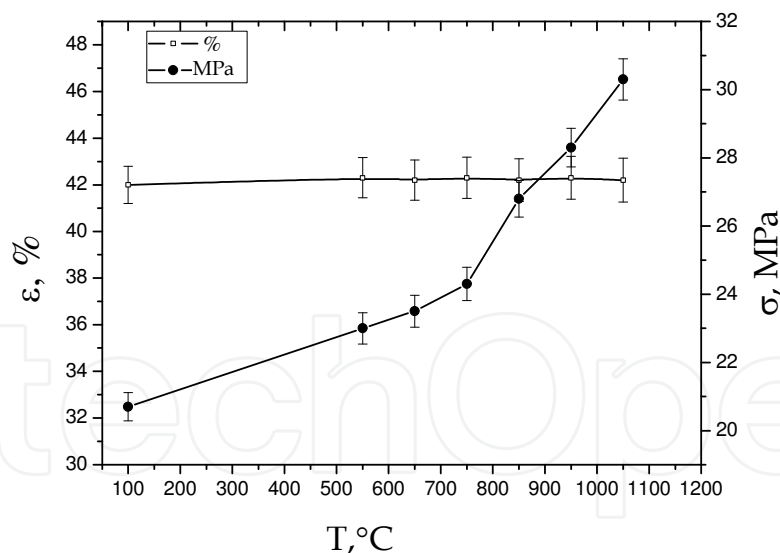
Fig. 4. Dependence of porosity ( \varepsilon ) and crushing strength ( \sigma ) on the calcination temperature for \text{Al}_2\text{O}_3/\text{Al} composite prepared from PAP-2.
