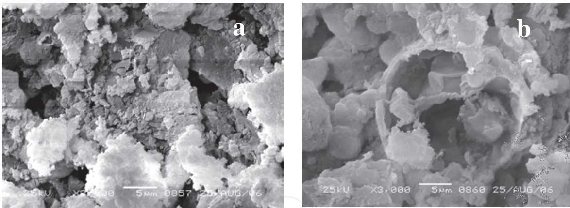
Fig. 10. SEM micrographs of the fracture surface of \text{Al}_2\text{O}_3/\text{Al} composite granules prepared from powdered TCA and PA-4.
