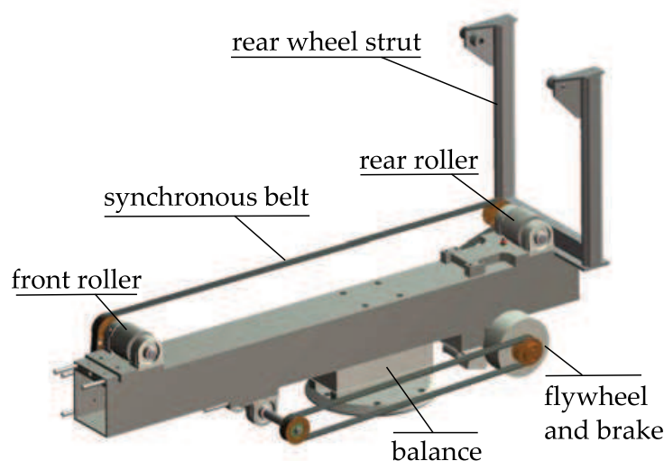
Fig. 7. The test rig for the cyclist
