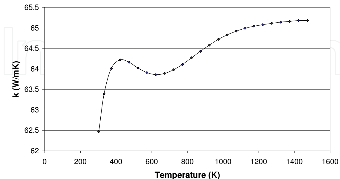
Fig. 4. UHTC Thermal conductivity vs Temperature
