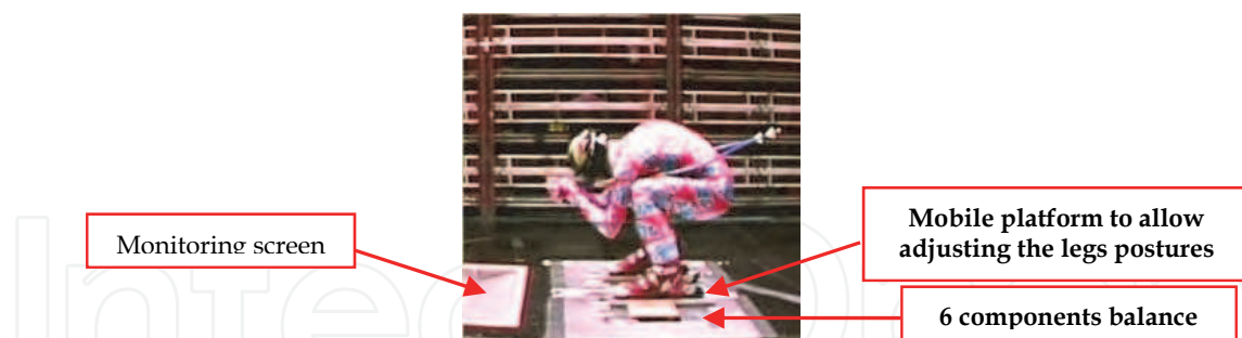
Fig. 15. Measuring device for the assessment of the drag applied on a downhill skier (Wind tunnel of IAT, France).
