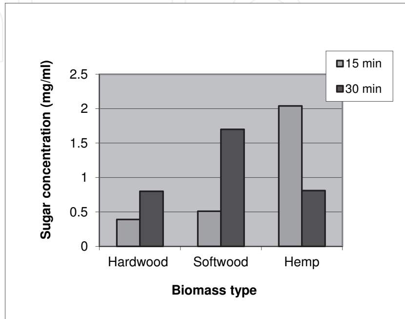
Fig. 7. Pretreatment of the biomass with H_2SO_4 1.23% at 120^\circ C
