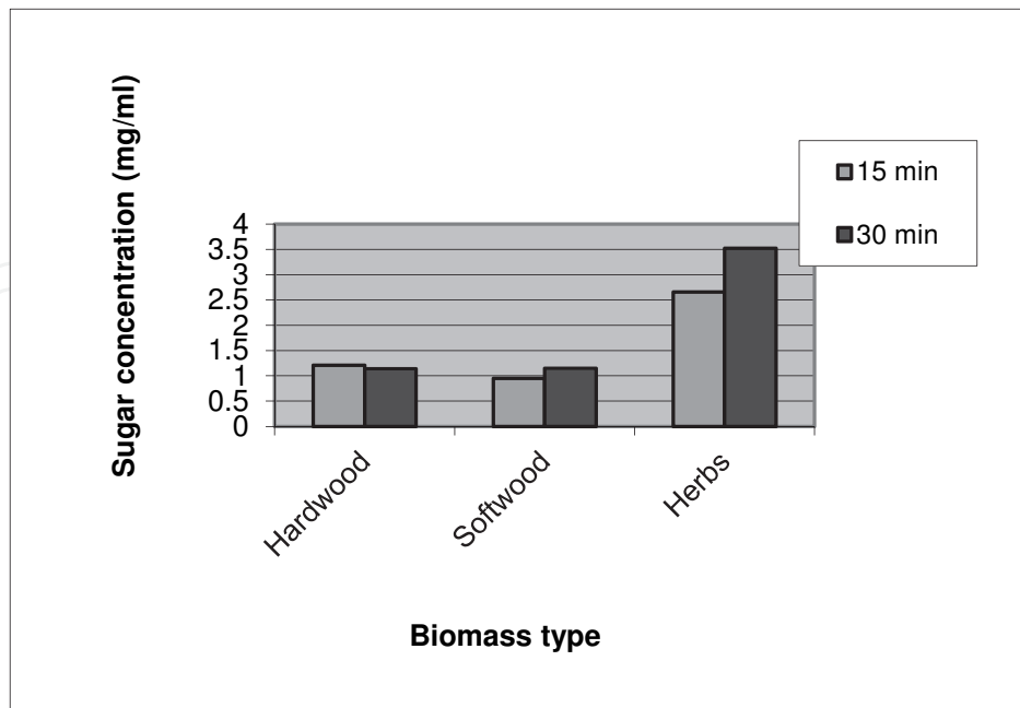
Fig. 10. Pretreatment of the biomass with H_2SO_4 1.64% at 120^\circ C
