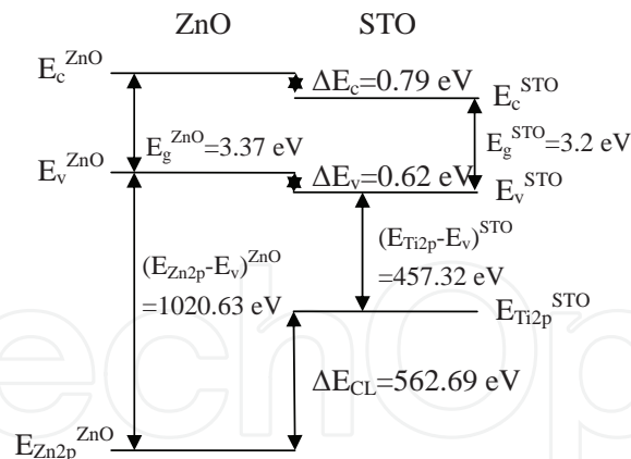
Fig. 4. Energy band diagram of ZnO/STO heterojunction.
