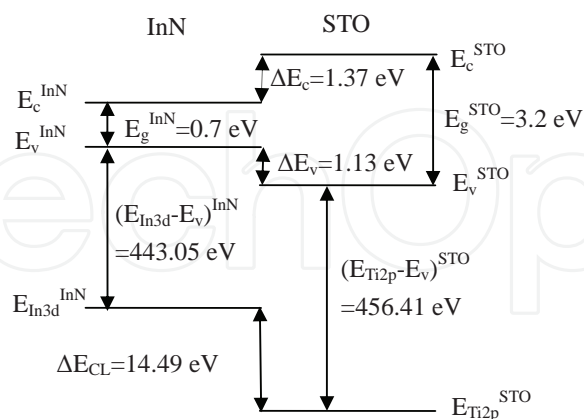
Fig. 10. Energy band diagram of InN/STO heterojunction.
