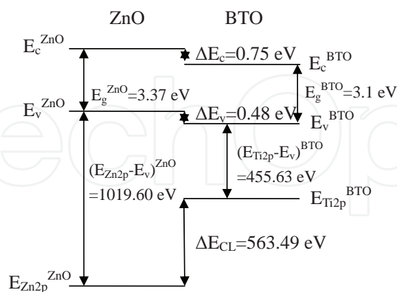
Fig. 7. Energy band diagram of ZnO/BTO heterojunction.
