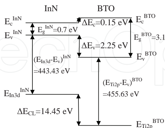
Fig. 13. Energy band diagram of InN/BTO heterojunction.
