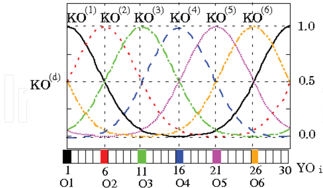
Fig. 4. Teaching signal for orientation recognition.
