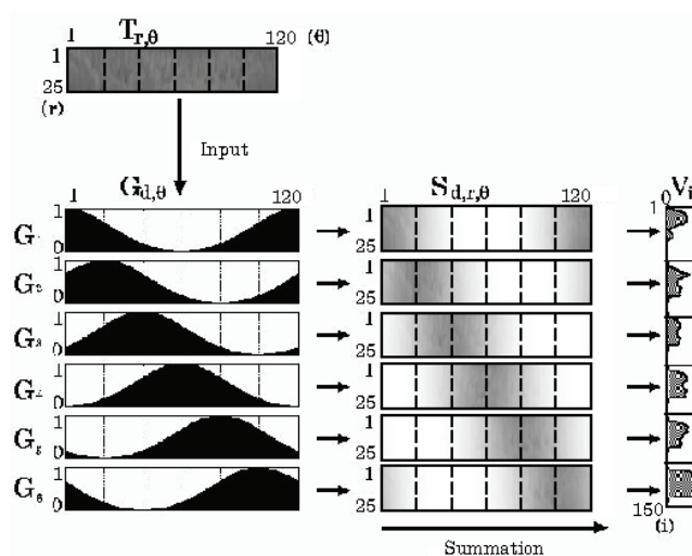
Fig. 3. Structure of the spreading layers.
