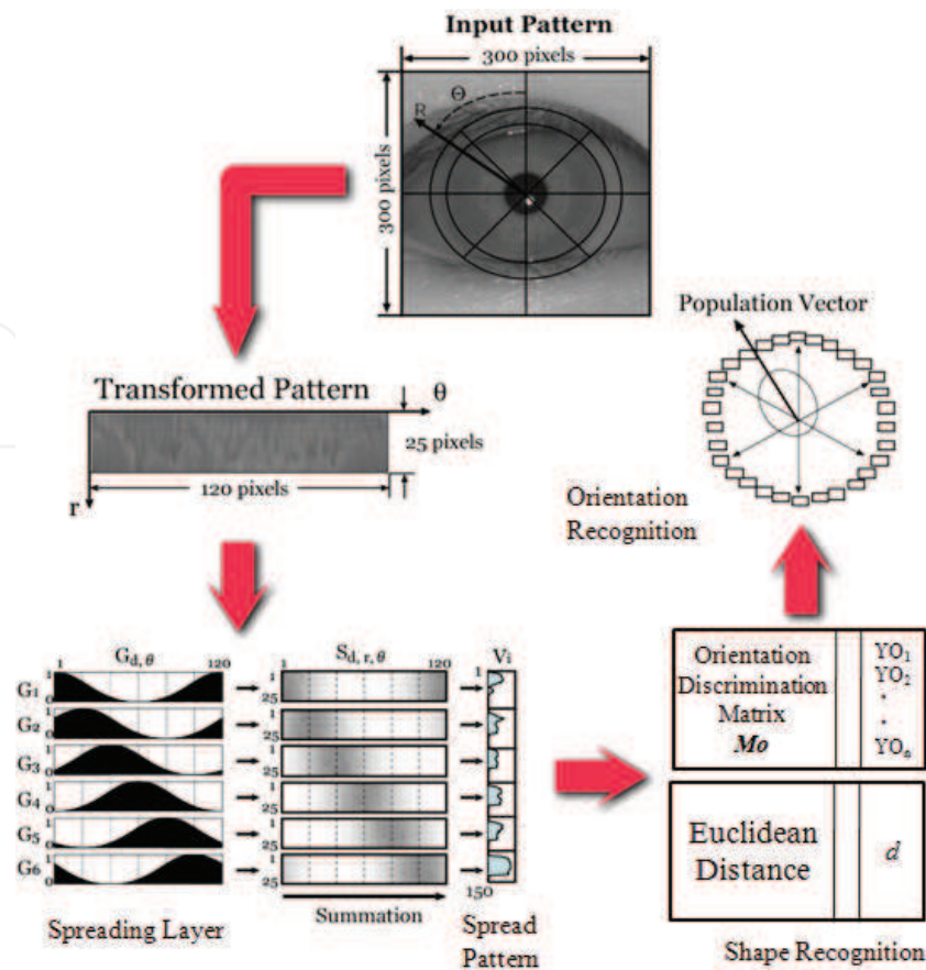
Fig. 1. Structure of the R-SAN net.
