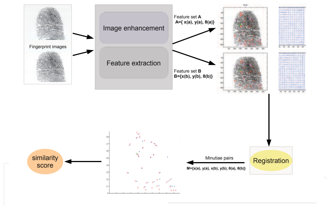
Fig. 4. General processes for minutiae-based fingerprint matching.
