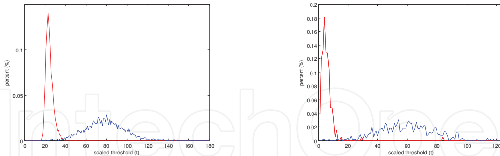
Fig. 16. Genuine (blue) and imposter (red) distributions for the left: FVC2002 Db1 set A database, and right: University of Bologna database.
