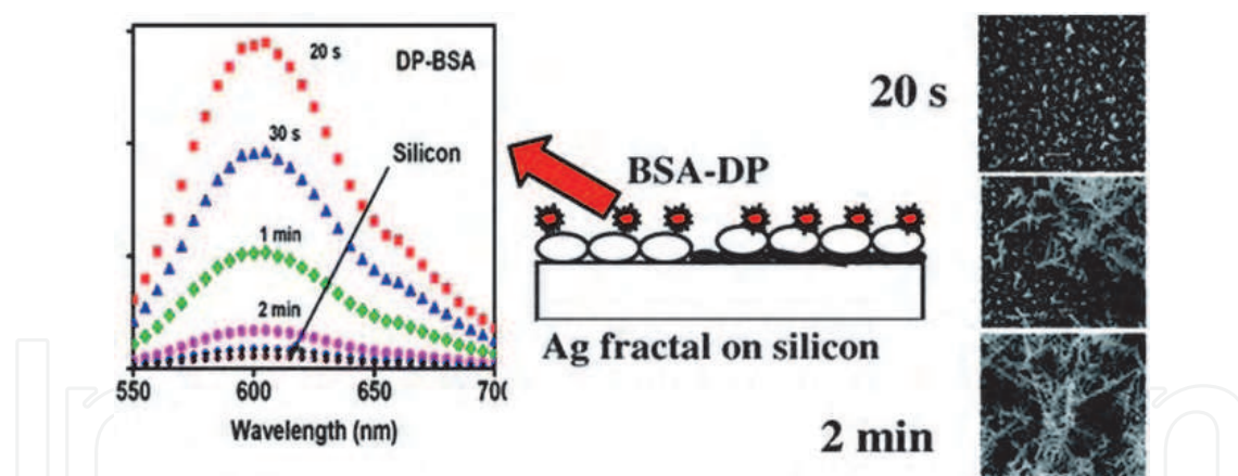
Fig. 7. Fluorescence enhancement study of BSA-Deep Purple (DP) fluorophore conjugate on silver fractal deposited by electroless deposition on silicon. Left: fluorescence spectra of DP for various silver growth times, middle: schematic of experimental sample, right: SEM images of silver fractals at various growth times. Reproduced from Ref (Drozdowicz-Tomsia et al 2010).
