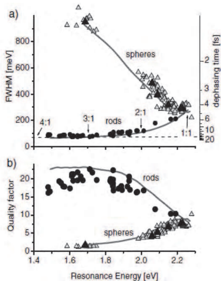
Fig. 3. (a) Measured linewidth ( G ) of plasmon resonances in single nanorods (dots) and nanospheres (open triangles) as a function of resonance energy E_{res} . The right scale gives the dephasing times calculated from G . Black triangles: averages for spherical particles of the same nominal size (150, 100, 80, 60, 40, and 20 nm from left to right). Lines: theoretical simulations. Some selected aspect ratios b/a are indicated in the figure. (b) The same data plotted as quality factor Q = E_{res}/G which is expressed as a ratio of extinction intensity at resonance to FWHM of plasmon peak. Reprinted from Ref (Sonnichsen et al 2002).
