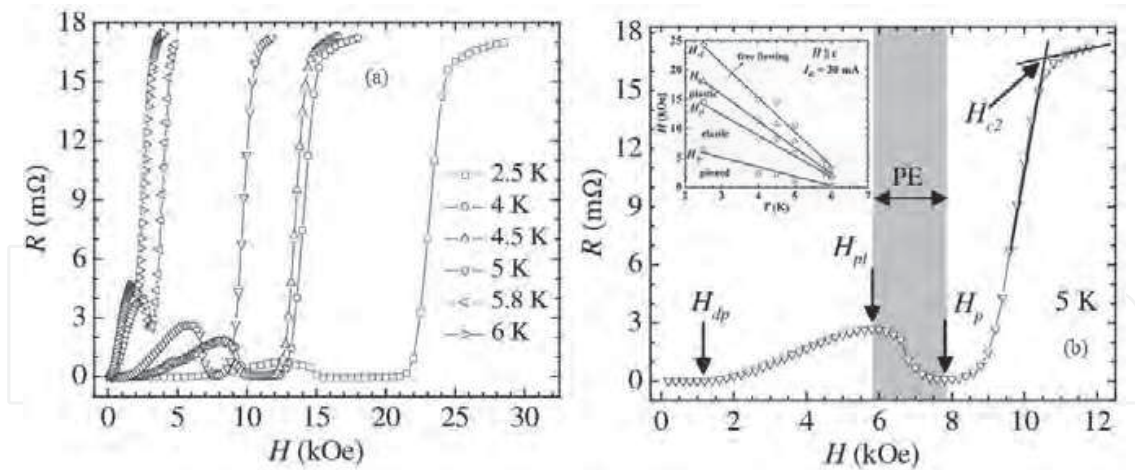
Fig. 10. (a) R versus H ( H \parallel c ) of the vortex state, measured at different T with I_{dc}=30 mA. (b) R-H at 5 K only, with the different driven vortex state regimes marked with arrows. The arrows marks the locations of, depinning ( H_{dp} ), onset of plastic deformations ( H_p ), peak location of PE ( H_p ) and upper critical field ( H_{c2} ) at 5 K, respectively. The inset location of above fields (Fig.10(b)) on the H-T diagram. [Mohan et al. 2009a; Mohan 2009b].
