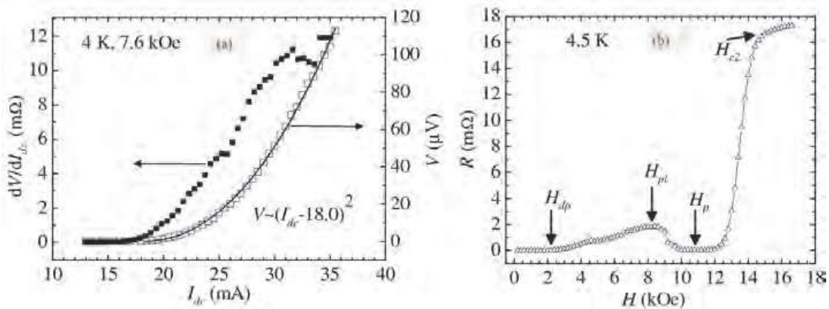
Fig. 11. (a) The V-I_{dc} characteristics and dV/dI_{dc} vs I_{dc} in the elastic phase at 4 K and 7.6 kOe. The solid line is a fit to the V-I_{dc} data, (cf. text for details). (b) R-H curve at 4.5 K and I_{dc}= 30 mA. [Mohan et al. 2009a; Mohan 2009b]
