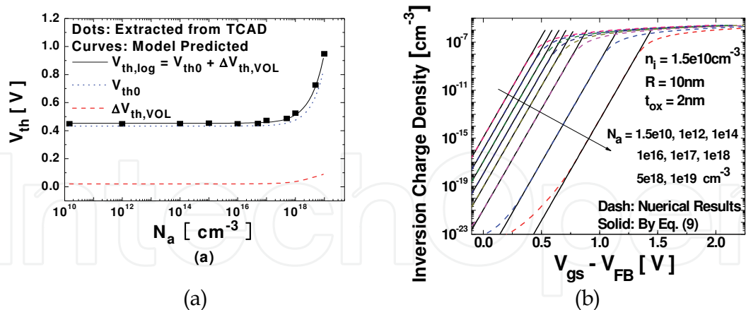
Fig. 34. (a) V_{th} model is compared with TCAD extracted by second derivative method in a long channel SNWT (From Yang J., IEEE TED, Vol. 55, No. 11, Nov. 2008)
