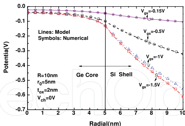
Fig. 28. Potential distribution along the radial of a Ge/Si core/shell structure. The lines denote results obtained from the analytic model and the symbols are results from numerical simulation (Zhang L. IEEE TED, Vol. 55, No. 11, Nov. 2008)
