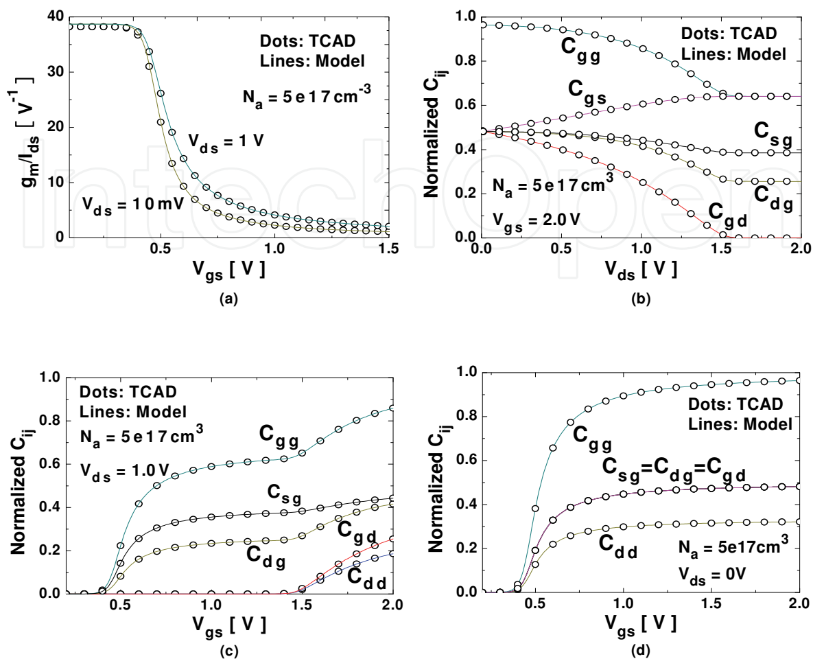
Fig. 37. ac characteristics verification of the model for a long channel SNWT (a) gm-efficiency, (b) C-Vds, (c) C-Vgs (at Vds≠0) and (d) C-Vgs (at Vds=0) (From Yang J., IEEE TED, Vol. 55, No. 11, Nov. 2008)
