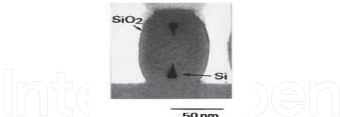
Fig. 7. Twin KOH based Multiple Silicon Nanowire (From Hideo Namatsu, J. Vac. Sci. Technol. B , Vol.15, No.5)
