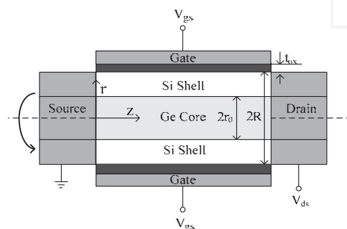
Fig. 26. Schematic diagram of a Ge/Si core/shell NWFET
