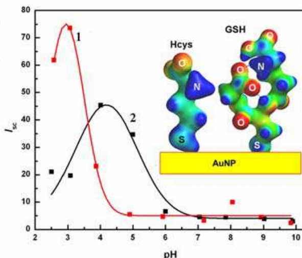
Fig. 6. Dependence of I_{sc} on pH for: (1) 20 \mu\text{M} GSH solutions and (2) 20 \mu\text{M} Hcys solutions; \tau = 60\text{s} ; C_{\text{AuNP}} = 3.8 \text{ nM} ; AuNP diameter: 5 nm, C_{\text{Cit}} = 0.46 \text{ mM} .
