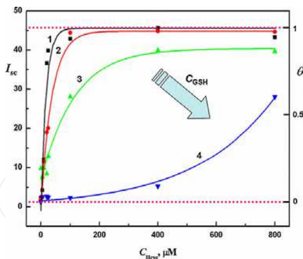
Fig. 7. Tuning the speed of ligand-exchange and SAM shell composition in fast AuNP functionalization; dependence of RELS intensity I_{sc} on C_{\text{Hcys}} for different C_{\text{GSH}} [ \mu\text{M} ]: (1) 5, (2) 20, (3) 100, (4) 400; C_{\text{AuNP}} = 3.8 \text{ nM} , citrate buffer, C_{\text{Cit}} = 0.46 \text{ mM} , \text{pH} = 5 , \lambda_{\text{ex}} = 640 \text{ nm} , \tau = 60 \text{ s} ; all curves are fitted with sigmoidal Boltzmann function.
