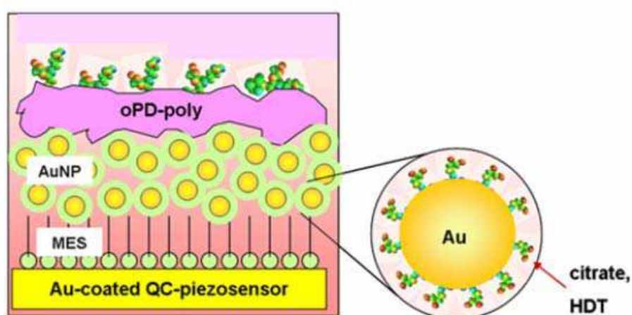
Fig. 8. Schematic of GSH-templated sensor design: GSH embedded in a PoPD film electrodeposited on a layer of AuNP network assembled on a SAM of MES on a Au piezoelector.
