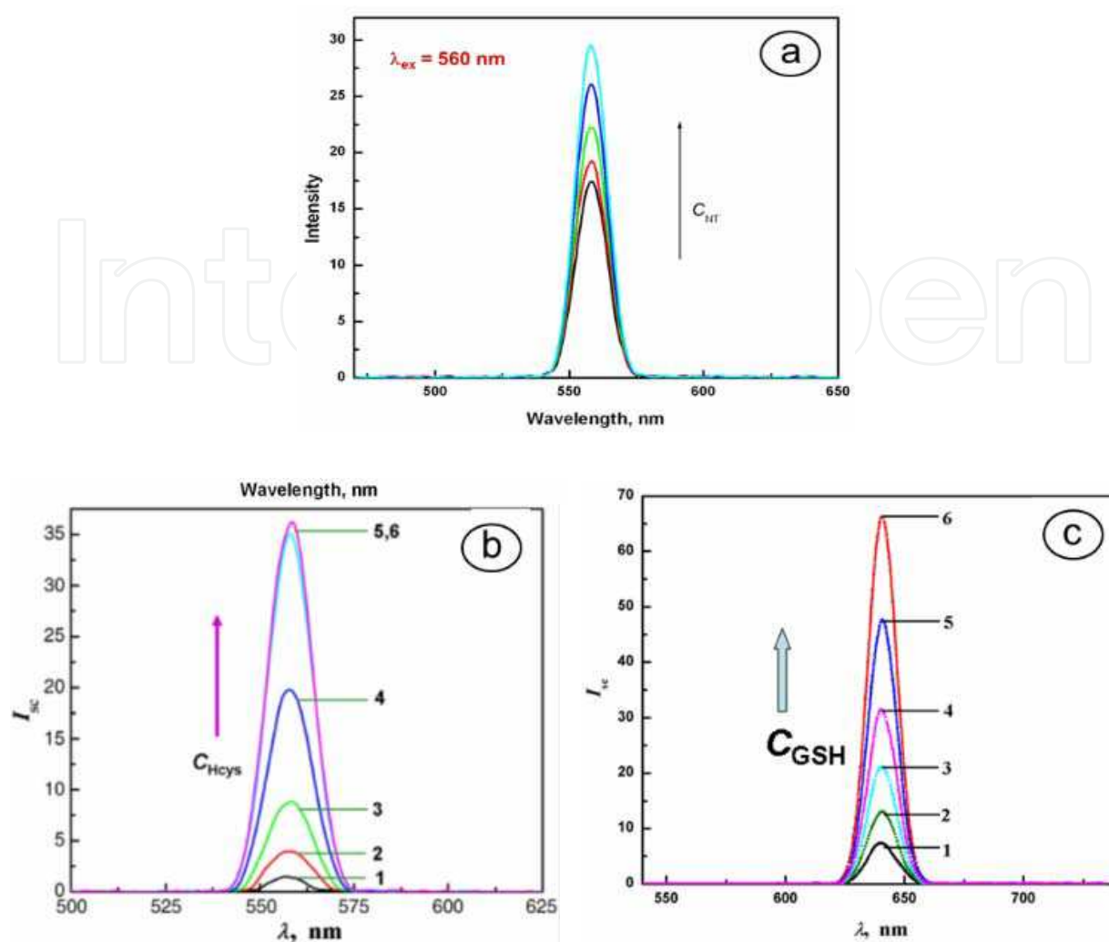
Fig. 4. (a) Dependence of RELS spectra for 0.95 nM cysteamine-capped AuNP 5nm + x \mu M NT, x [ \mu M]: (1) 0, (2) 83.3, (3) 166.7, (4) 250, (5) 333; \lambda_{\text{ex}} = 560 nm; 20 mM TrisHCl buffer, pH = 7.4; (b-c) Resonance elastic light scattering spectra for citrate-capped AuNP 5 nm for different concentrations of (b) homocysteine and (c) glutathione, C_{\text{Hcys}} [ \mu M]: (1) 0, (2) 5, (3) 5.5, (4) 5.75, (5) 6.75, (6) 15, C_{\text{AuNP}} = 3.8 nM, pH = 5, \lambda_{\text{ex}} = 560 nm; C_{\text{GSH}} [mM]: (1) 0, (2) 2.67, (3) 3.0, (4) 3.17, (5) 3.33, (6) 5, C_{\text{AuNP}} = 10.1 nM.
