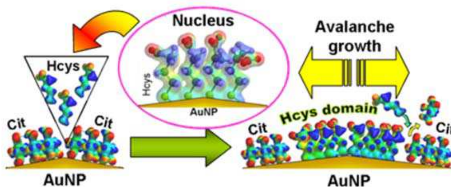
Scheme 2. Schematic view of the hydrogen bonded citrate SAM basal film and the nucleation and growth of a hydrogen bonded Hcys-ligand domain on an edge of a citrate-capped AuNP.
