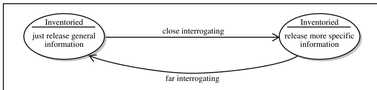
Fig. 8. Fishkin's approach
