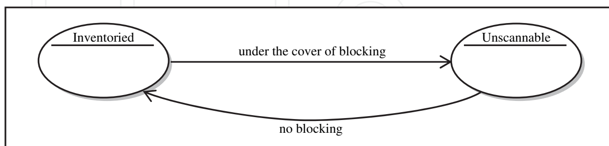
Fig. 9. Blocking approach
