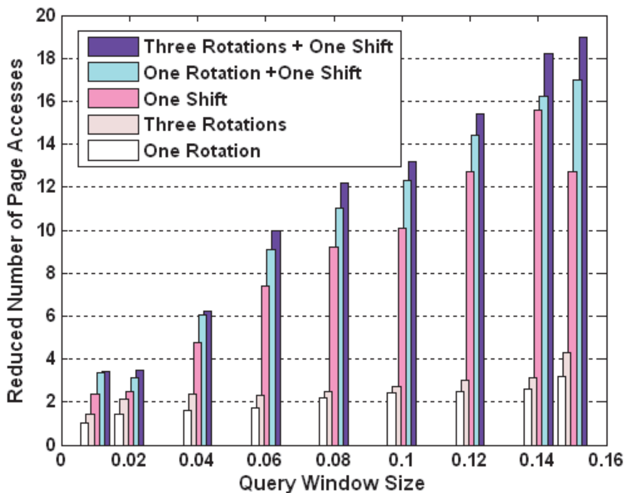
Fig. 10. Efficiency comparisons.
