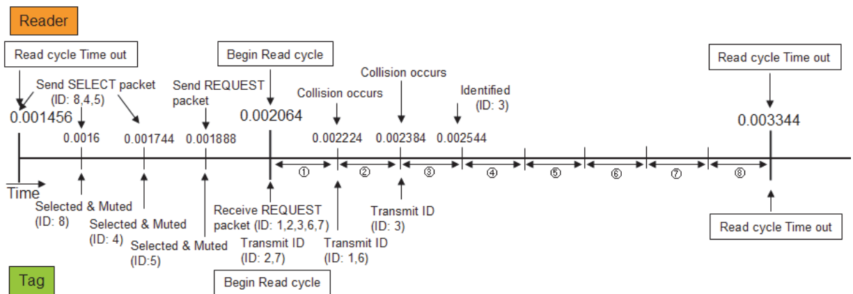
(b) Second Read Cycle of the Simulation
