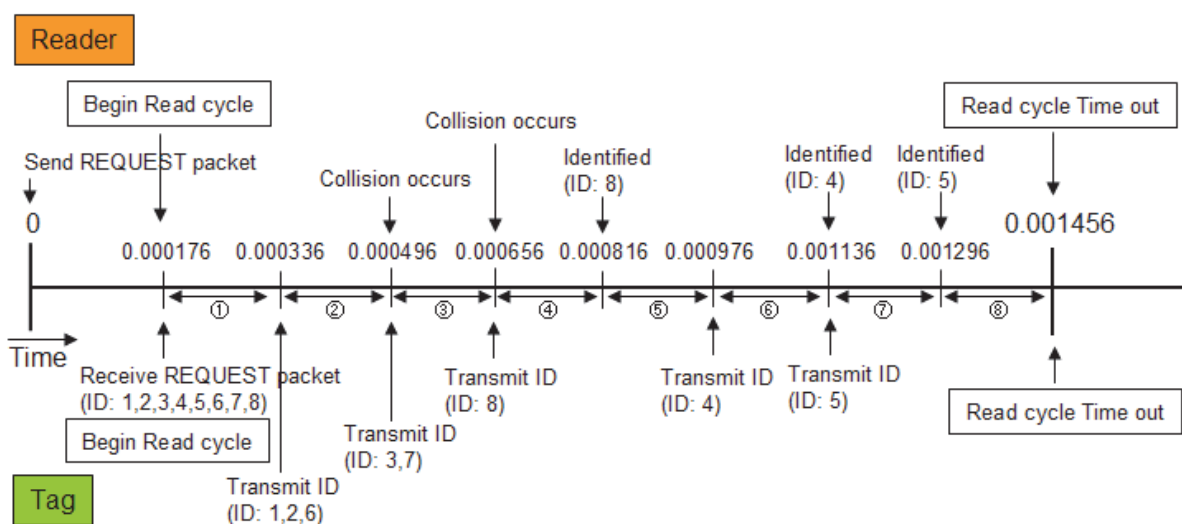
(a) First Read Cycle of the Simulation
