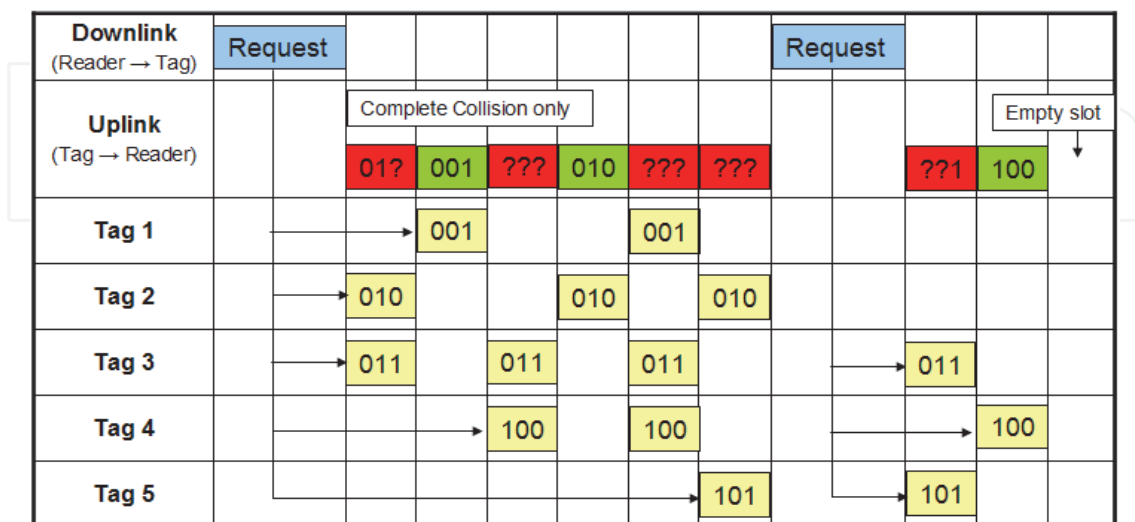
(b) Slotted ALOHA
