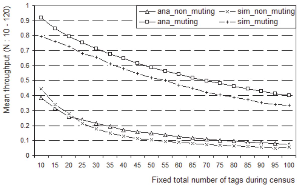
(c) Mean Network Throughput
