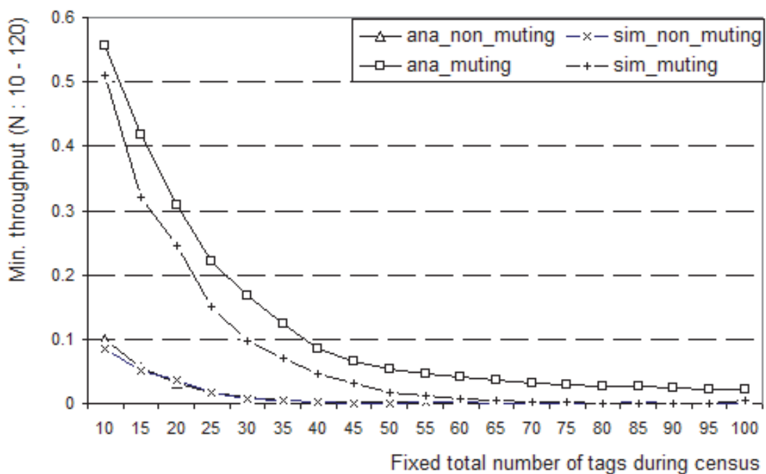
(a) Minimum Network Throughput
