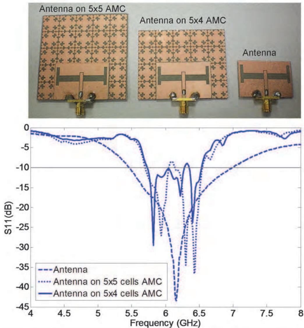
Fig. 6. Manufactured prototypes of the antenna on 5x5 cells AMC, the antenna on 5x4 cells and the antenna (up). Return loss of the Antenna, the antenna on 5x5 cells AMC and the antenna on 5x4 cells (down).
