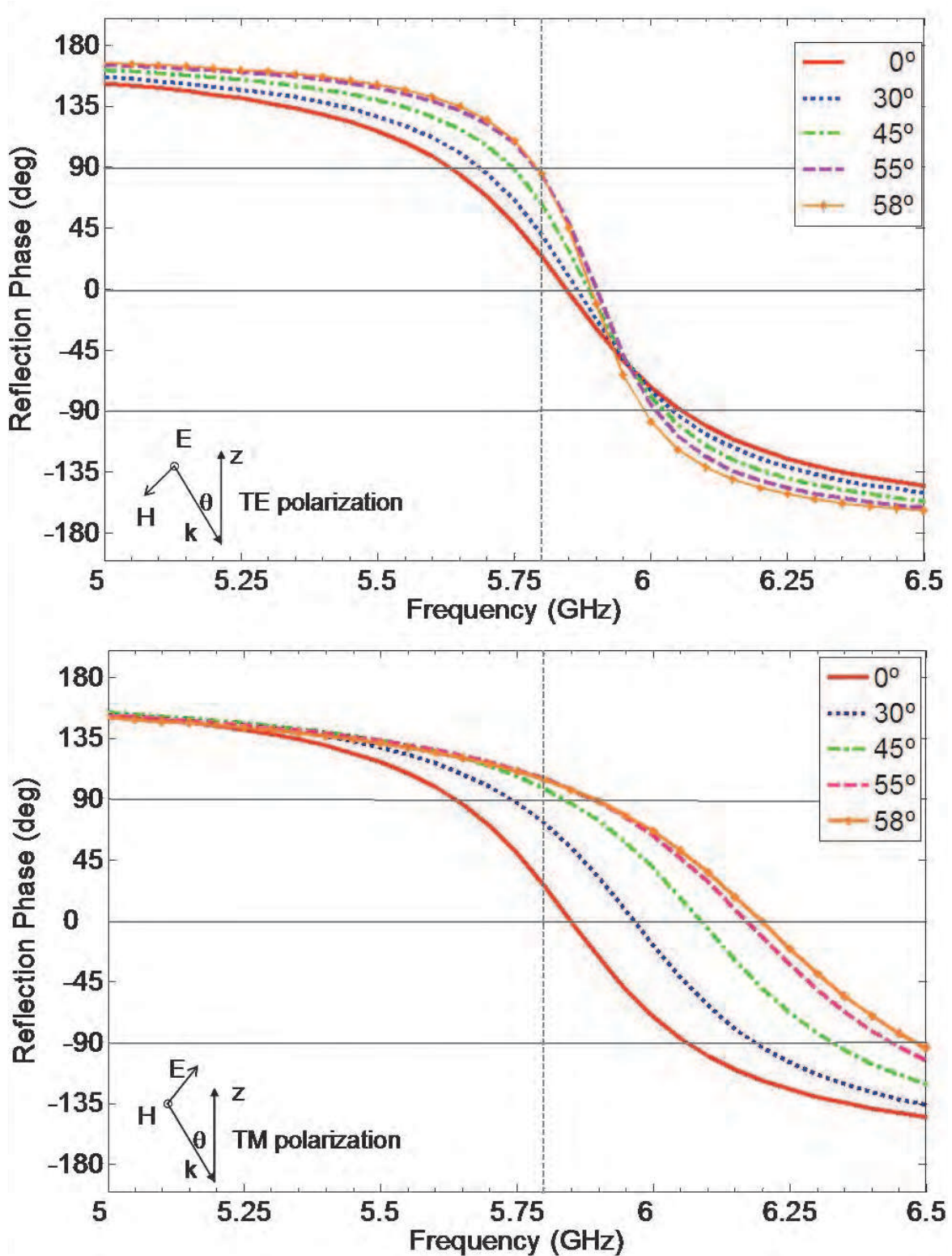
Fig. 3. Simulated Reflection phase of the AMC surface for TE (up) and TM (down) polarizations for different incident angles \theta_{inc}=0^\circ, 30^\circ, 45^\circ, 55^\circ and 58^\circ .
