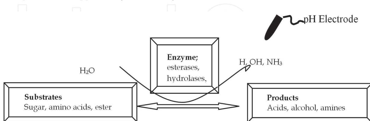
Fig. 3. Principle of working of a potentiometric sensor for the analysis of amino acids, sugars and esters. The enzymes are immobilized at the pH-electrode surface and the change in pH caused due to enzymatic conversion of the substrate is recorded, which is proportional to analyte concentration.
