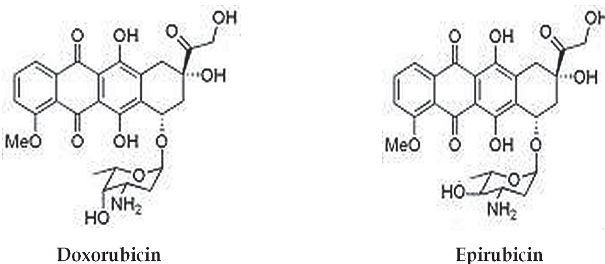
Fig. 4. Chemical structures of doxorubicin and doxorubicin
