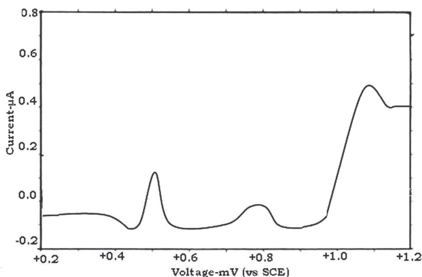
Fig. 9. Differential Pulse Voltammogram in 0.1\text{M} acetate buffer at \text{pH } 4.5 \pm 0.1 obtained with a thick later ds-DNA modified GCFE after being immersed in 20\mu\text{g/ml} epirubicin solution for 60 s at potential -0.60\text{V} .
