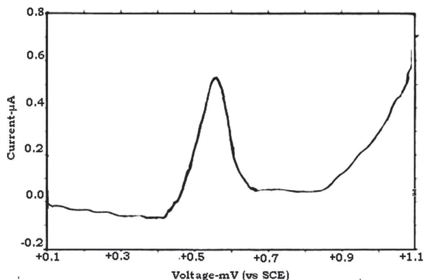
Fig. 6. Differential Pulse Voltammogram for 80 \mu g/ml epirubicin (oxidation) in 0.1M acetate buffer at pH 4.5 \pm 0.1 at bare GCFE.
