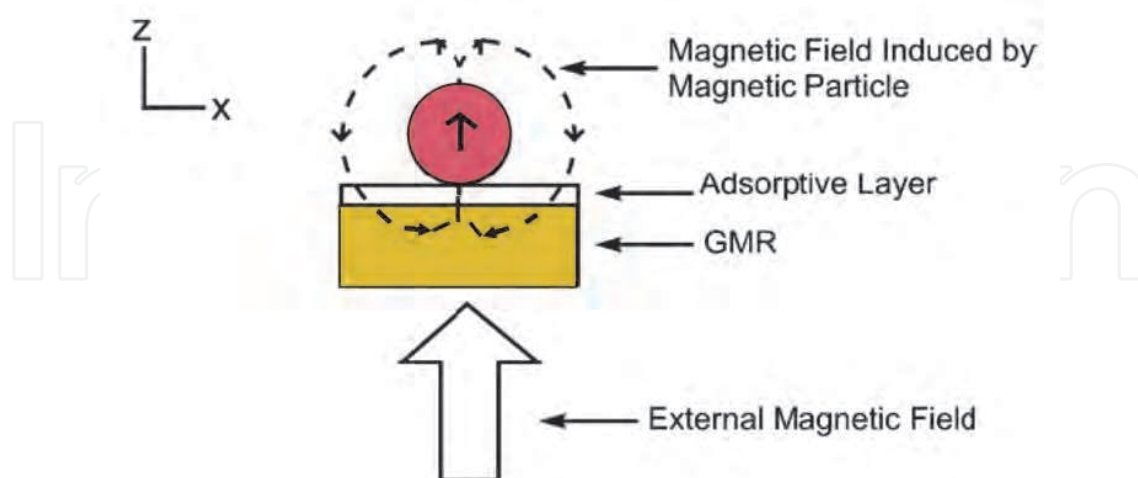
Fig. 14. Detection of magnetic particle on GMR biosensor (Adapted from Rife et al., 2003).
