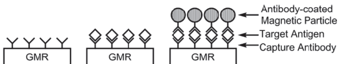
Fig. 13. Bacteria sensing using a GMR biosensor (Adapted from Millen et al., 2005).
