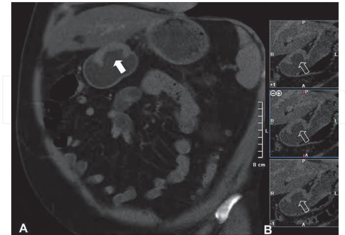
Fig. 4. Gastric ulcerative carcinoma. Same patient as in Fig. 3. A. CT reconstruction on oblique coronal plane. The tumor appears as an ulcerating wall thickening (arrow). B. Vessel Probe reconstructions allow to obtain a better identification of the gastric wall in the lesion site (empty arrows).
