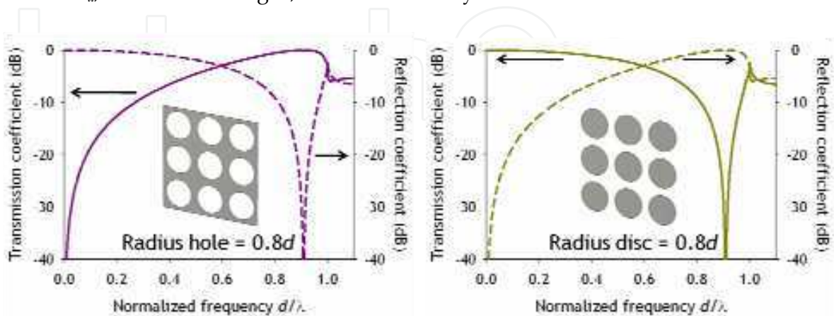
Fig. 6. Scattering parameters in logarithm scale of hole (left) and disk arrays (right) under vertically polarized illumination. (solid line) Transmission coefficient and (dashed line) reflection coefficient
