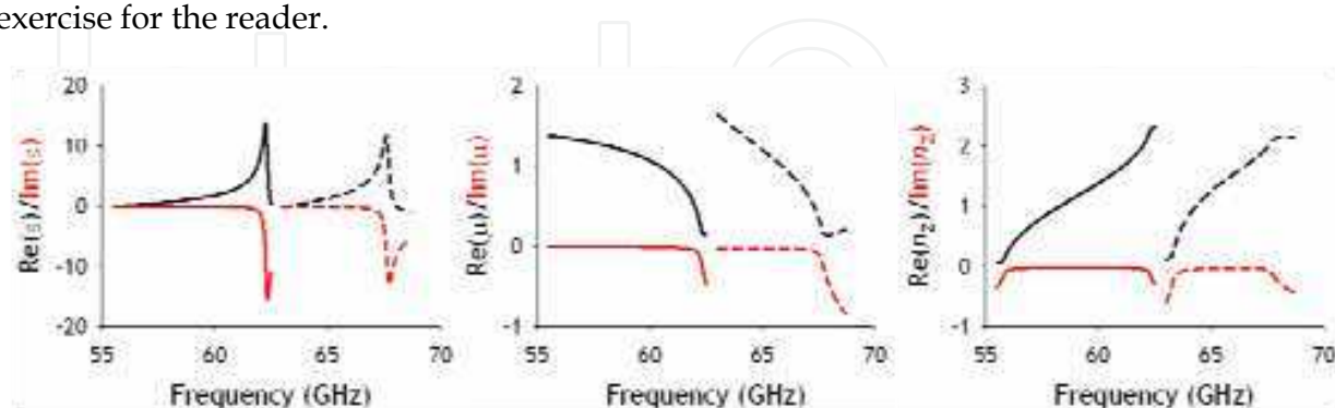
Fig. 13. From left to right: effective electric permittivity, magnetic permeability, and index of refraction. Solid and dashed lines account for E_y (vertical) and E_x (horizontal) polarization, respectively. Black and red lines represent real and imaginary part of the aforementioned constitutive parameters, respectively. The values are only computed within the -3 dB pass-band
