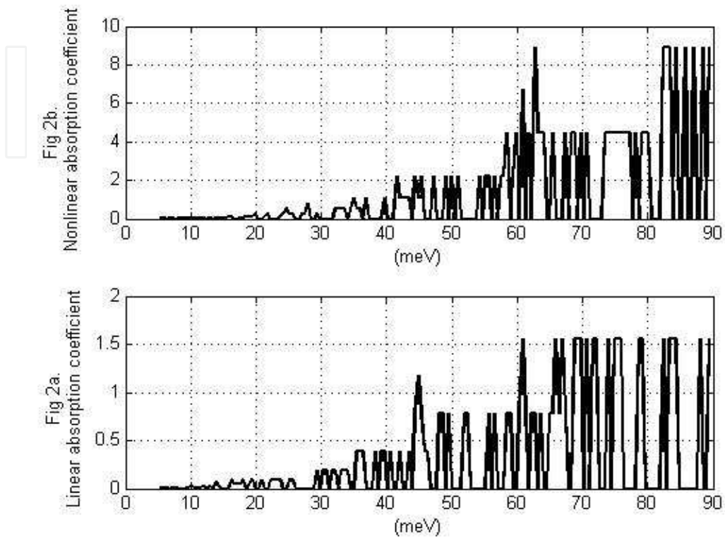
Fig. 2. The dependence of absorption coefficient on \hbar\Omega_B in case of confined phonons
