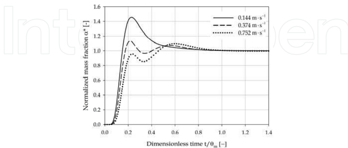
Fig. 7. Tracer response curve for different tip speeds at a point near the upper stirrer in the UniVessel 2L single-use. For better comparison, time is given as dimensionless
