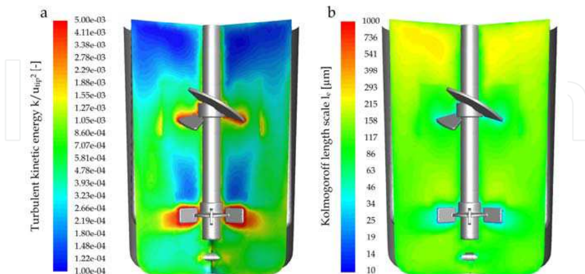
Fig. 11. Spatial distributions of the dimensionless turbulent kinetic energy k/u_{tip}^2 (a) and the Kolmogorov eddy size l_e (b) at P/V = 230 \text{ W}\cdot\text{m}^{-3} in the UniVessel® 2L single-use
