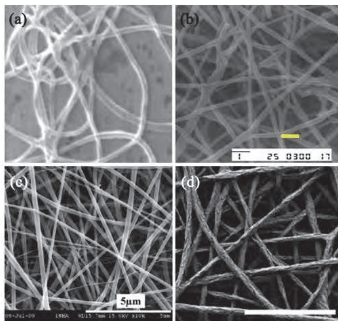
Fig. 6. SEM Image of (a) polyaniline fibers with an average diameter of 139 nm, (MacDiarmid et al., 2001), (b) polypyrrole/PEO composite nanofibers (the scale bar is 1 \mu\text{m} ), (Chronakis et al. 2006), (c) PEDOT:PSS/PVP nanofibers (Choi et al., 2010), and (d) PEDOT nanofibers fabricated using a combination of electro-spinning and vapor-phase polymerization (the scale bar is 5 \mu\text{m} ) (Laforgue & Robitaille, 2010).
