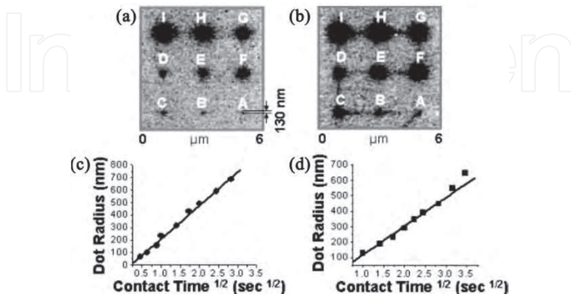
Fig. 8. Diffusion properties of conducting polymers on modified silicon substrates. Lateral force microscopy (LFM) images of (a) SPAN dots and (b) polypyrrole dots as a function of tip-substrate contact time. (c) Plot of the feature radius as a function of t^{1/2} for SPAN and (d) polypyrrole (Lim & Mirkin, 2002).
