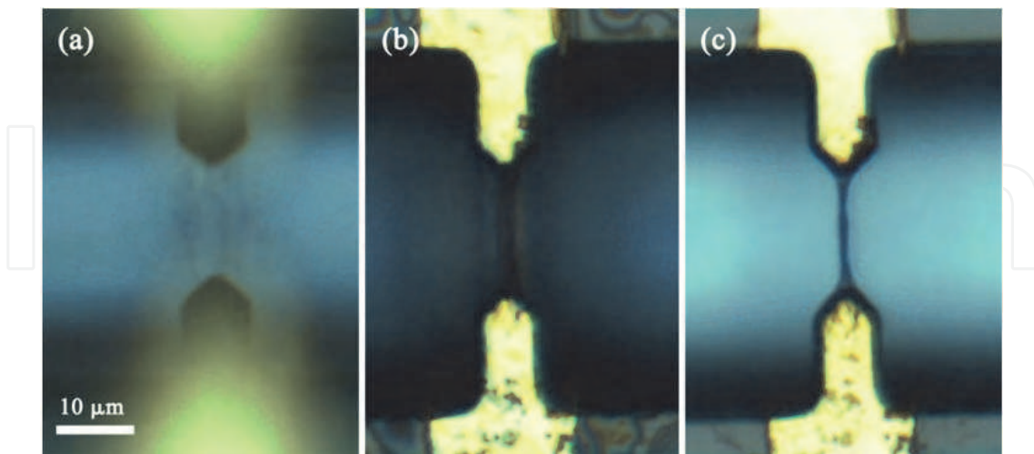
Fig. 12. Microscope images of the CNT-conducting polymer nanowire fabrication process using dielectrophoresis. (a) Attraction of the CNT and monomer molecules between electrodes with an AC electric field; (b) Compression of the CNT and monomer by suspension evaporation; (c) A CNT-conducting polymer nanowire synthesized between electrodes.
