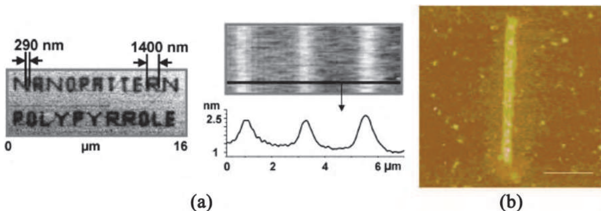
Fig. 9. (a) LFM (left) and topography (right-top) images of polypyrrole lines and the cross-sectional profile (right-bottom) (Lim & Mirkin, 2002). (b) PEDOT line patterned on \text{SiO}_2 . Polymer line width: 200 nm; scale bar: 1 \mu\text{m} (Maynor et al., 2002).
