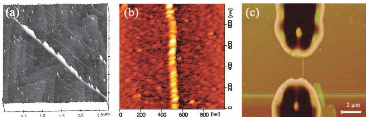
Fig. 5. AFM images of DNA/conducting polymer nanowires; (a) DNA/polypyrrole nanowire. The highlighted part is a DNA/polypyrrole nanowire and the others are bare DNA-scaffold molecules (Dong et al., 2007); (b) DNA/polypyrrole nanowire (Moon et al., 2010); (c) DNA/polyindole nanowires aligned between Au electrodes (Hassaniien et al., 2010).
