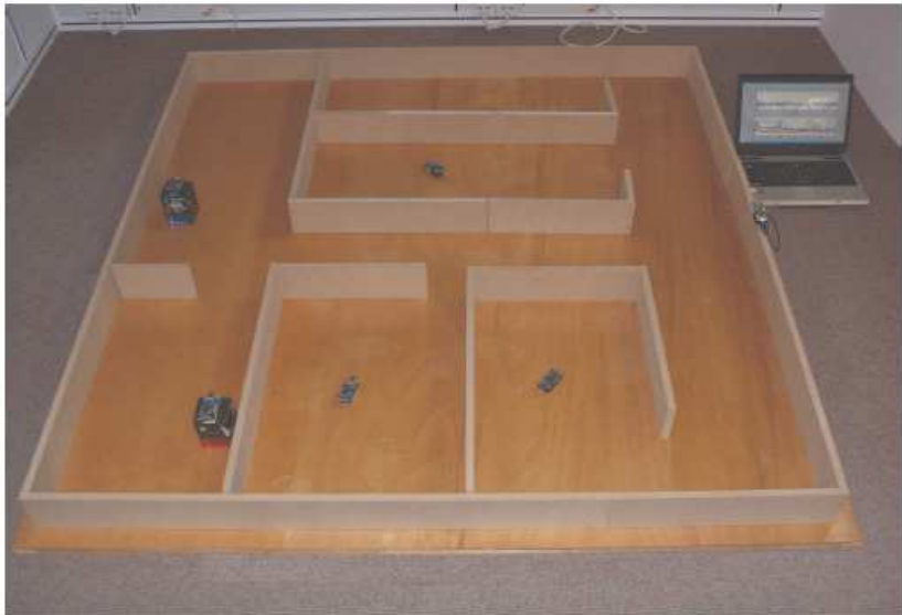
Fig. 19. Testbed Architecture
