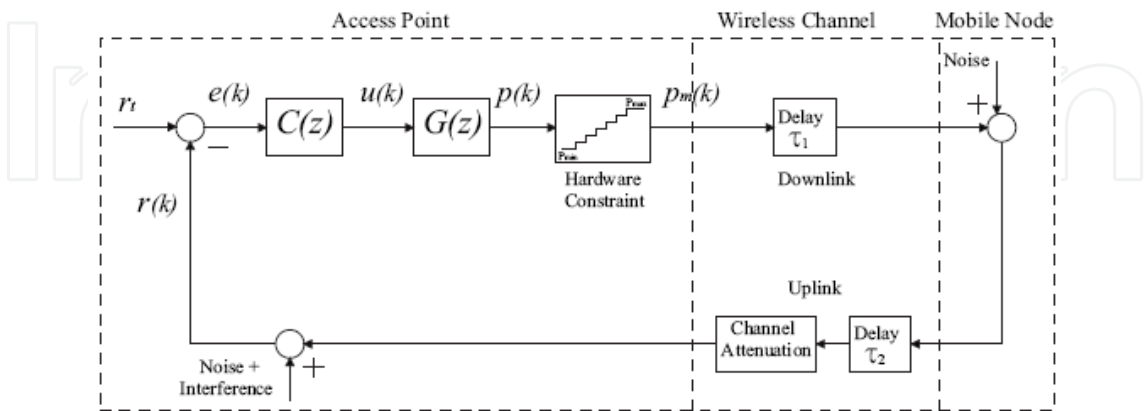
Fig. 3. Block diagram of the WSN Closed Loop Distributed Power Control structure based on RSSI measurement.
