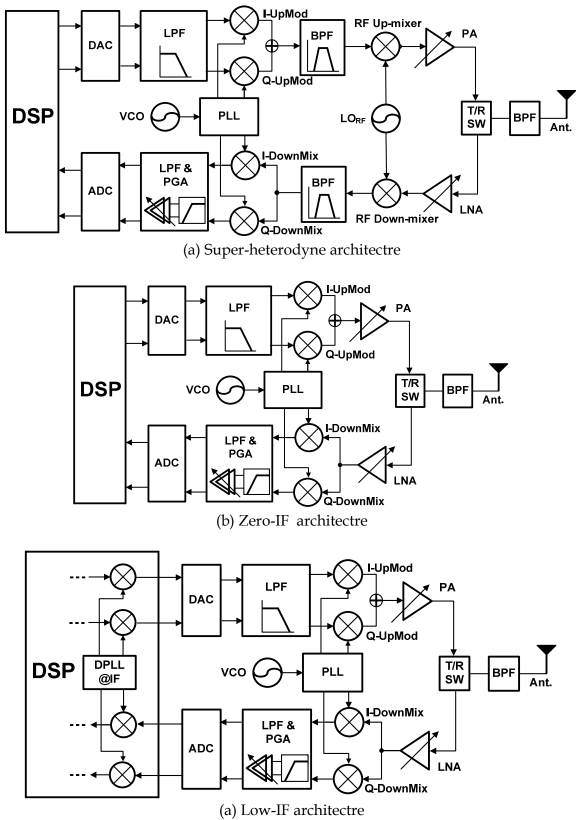
Fig. 1. Transceiver architectures
