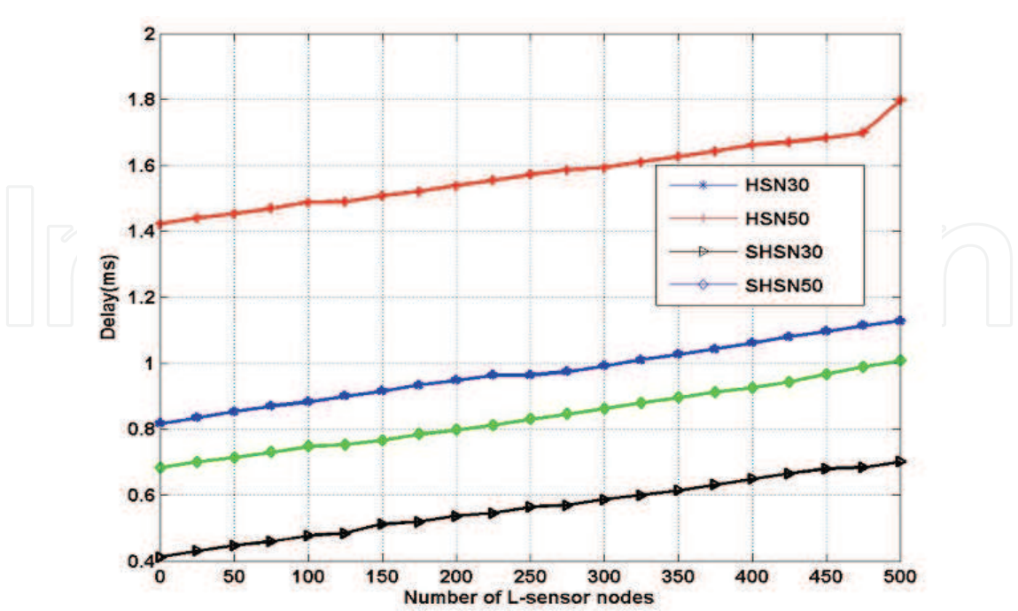
Fig. 19. Delay with respect to number of L-sensor nodes for coverage area 300m×300m
