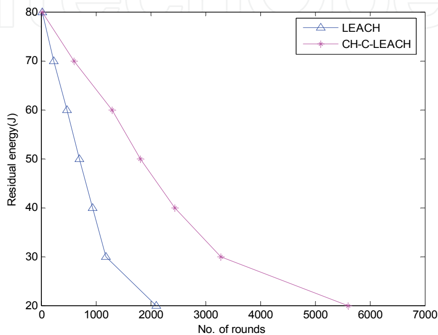
Fig. 6. Energy analysis of CH-C-LEACH scheme
