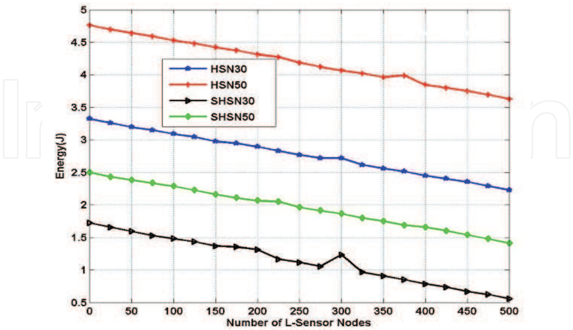
Fig. 17. Energy consumption with number of L- sensor nodes for coverage area 500m×500m
