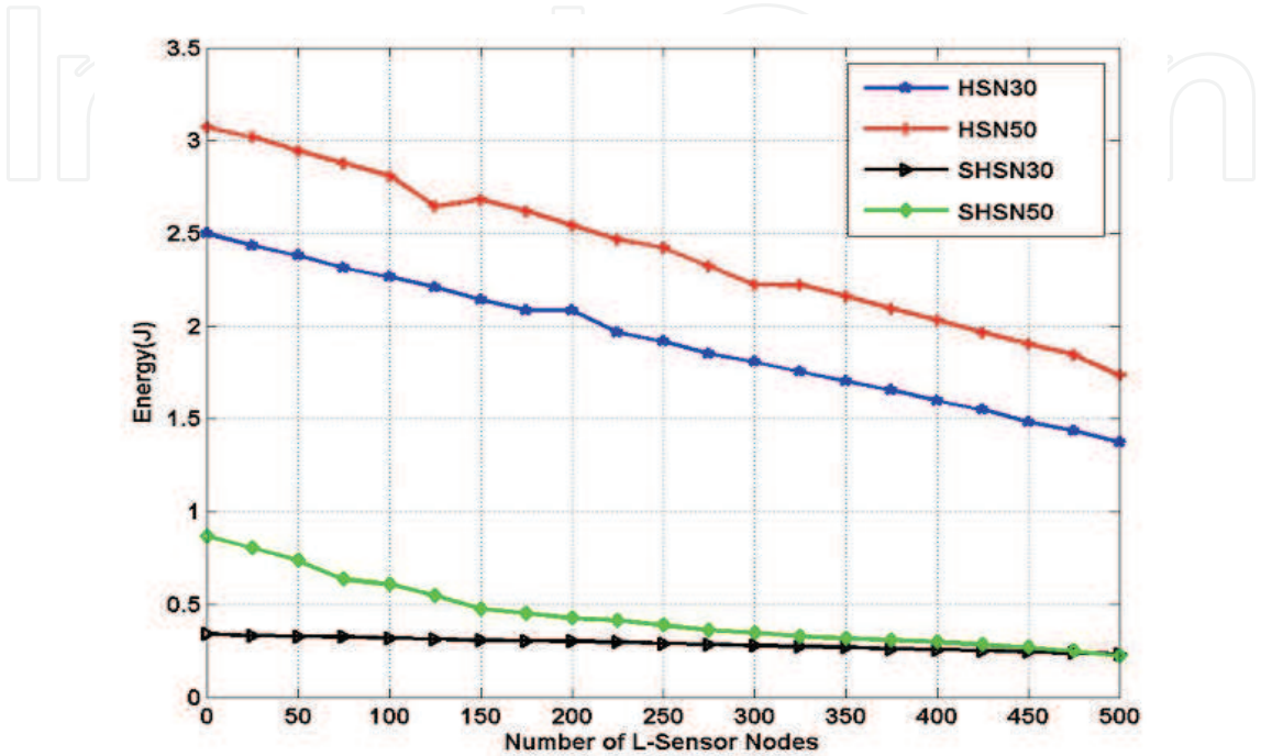
Fig. 16. Energy consumption with number of L-sensor nodes for coverage area 300m×300m
