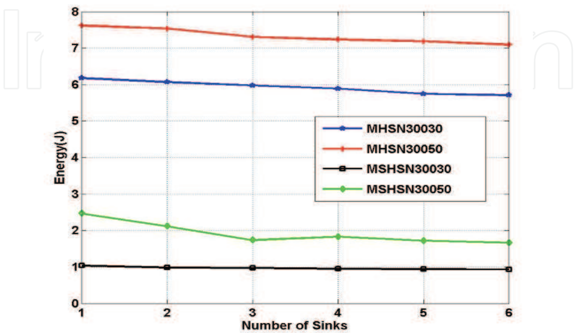
Fig. 18. Energy consumption with number of mobile sinks for coverage area 300m×300m
