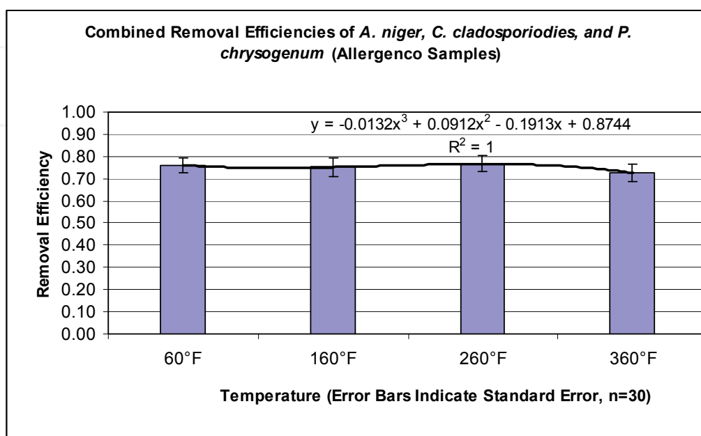
Fig. 20. Combined removal efficiencies of the Aspergillus niger , Cladosporium cladosporioides , and Penicillium chrysogenum –Allergenco Microbial Air Sampler data sets.
