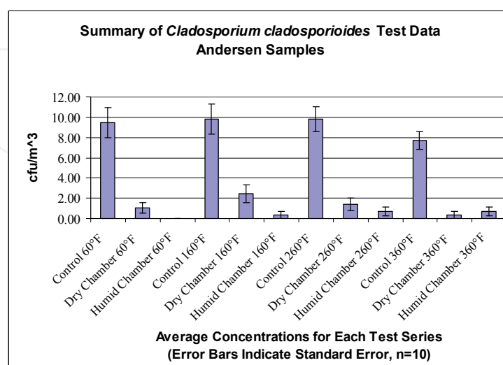
Fig. 8. Average airborne concentrations for Cladosporium cladosporioides -Andersen Impactor tests.
