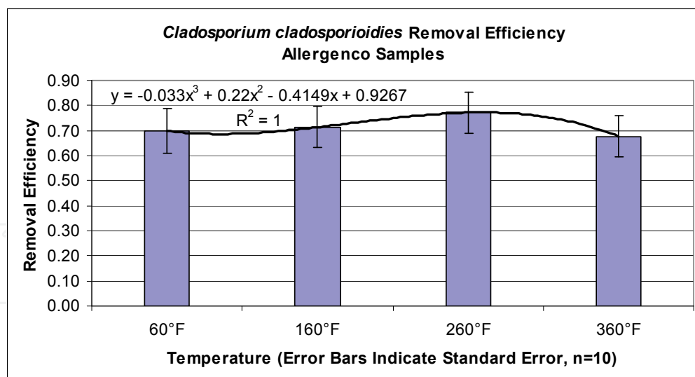
Fig. 17. Cladosporium cladosporioides Removal Efficiencies for Allergenco Samples.
