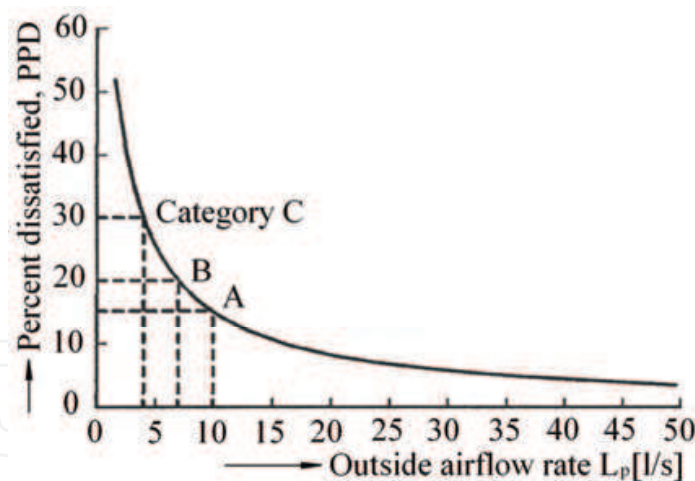
Fig. 5. PPD as a function of ventilation rate per standard person (i.e., per olf )
