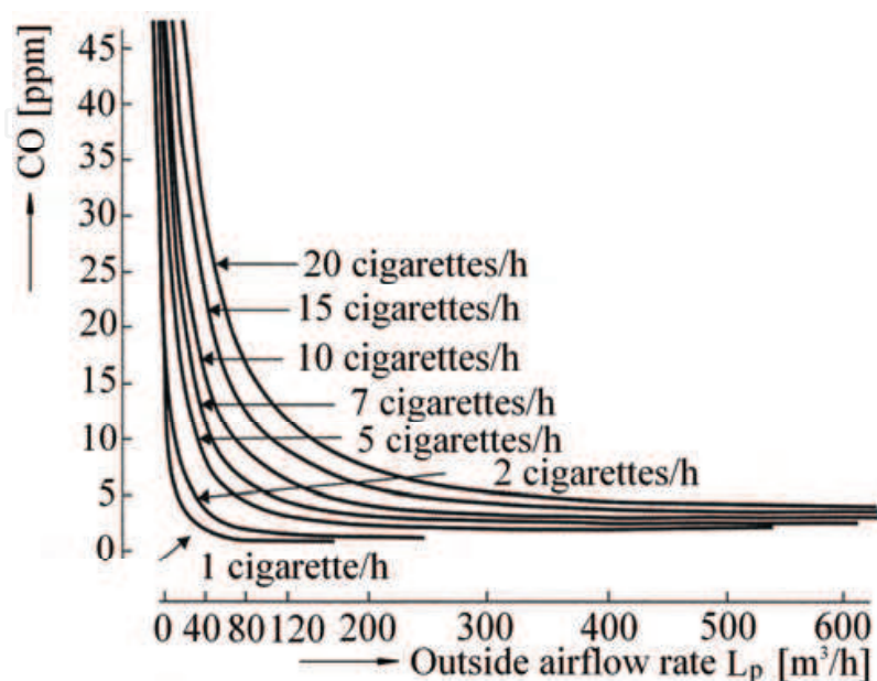
Fig. 4. Variation of CO concentration
