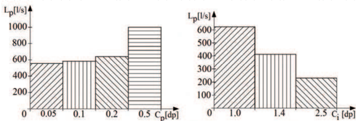
Fig. 10. Variation of outside air flow-rate function of outdoor and indoor air quality
