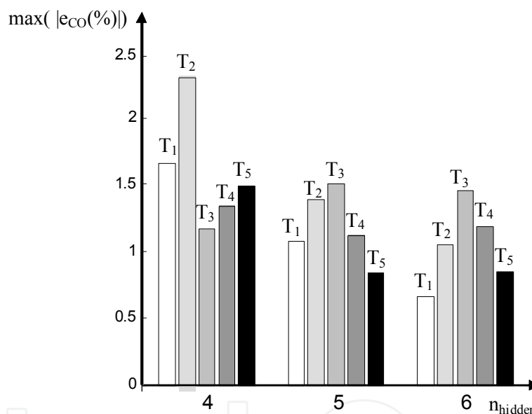
Fig. 8. The maximum inverse modeling error for different NPB CO architectures ( n_{\text{hidden}}=\{4, 5, 6\} ) and different temperatures T_p=10 \cdot p^{\circ}\text{C}
