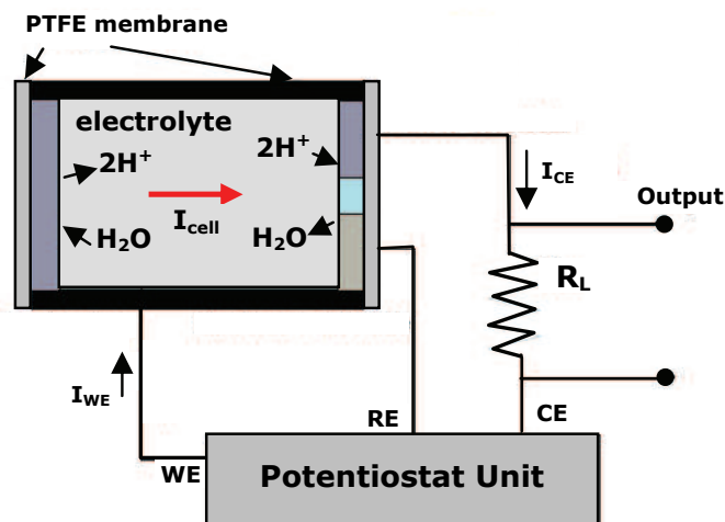
Fig. 2. Gas sensing unit based on an electrochemical cell ( RE - reference electrode, CE - counting electrode, WE - working electrode, R_L - load resistance)
