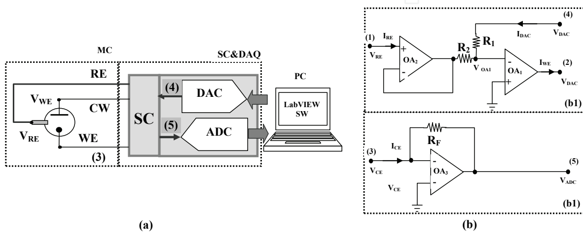
Fig. 3. Electrical circuit of a voltammetry measuring system (MS- measuring cell, RE- reference electrode, CE- counting electrode, WE- working electrode, SC&DAQ- signal conditioning and data acquisition, ADC- analogue to digital converter, DAC- digital to analog converter, OA- operational amplifier)
