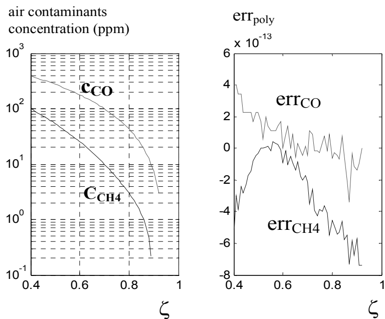
Fig. 5. Polynomial approximation of air contaminants curves (CO and methane case) and polynomial approximation error ( err_{CO} , err_{CH4} )
