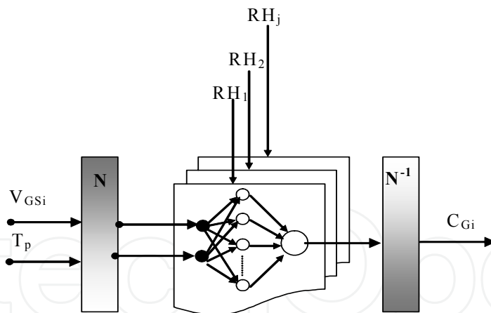
Fig. 6. NPB_i architecture ( N , N^{-1} : normalization and denormalization blocks; RH_j : humidity selector; C_{Gi} : temperature and humidity compensated values of G_i gas concentration; T_p : temperature input value, V_{GSi} : input voltage value on the GS_i channel).
