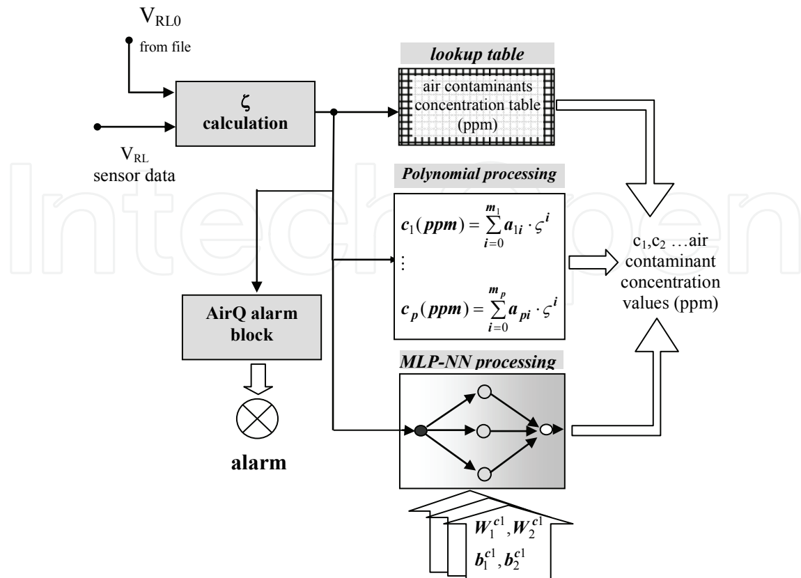
Fig. 4. Block diagram of the hybrid data processing scheme that was used to evaluate contaminants' air concentrations.
