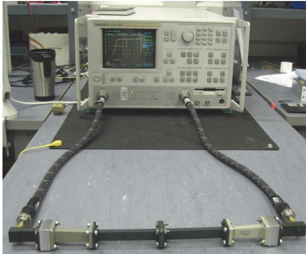
Fig. 8. A 20 cm rectangular waveguide connected to the VNA, via tapers, chokes, adapters, and coaxial cables.
