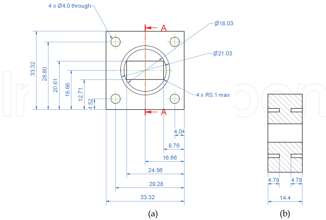
Fig. 6. Parameters of the (a) cross section and (b) side view of the choke.
