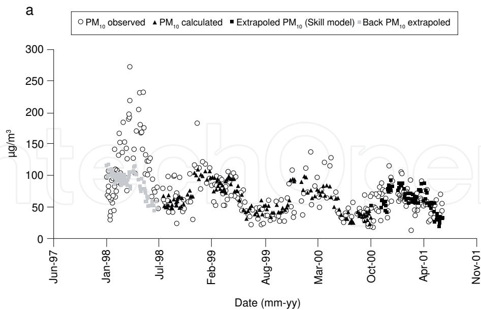
Fig. 2. Observed and estimated PM_{10} vs. date from January (1998) to June (2001). SWof MC. Higher values ( > 200 \mu\text{g m}^{-3} ) due to forest fires. Taken from Bravo et al. (2006).
