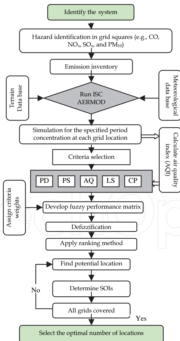
Fig. 2. Framework for designing AQMN
