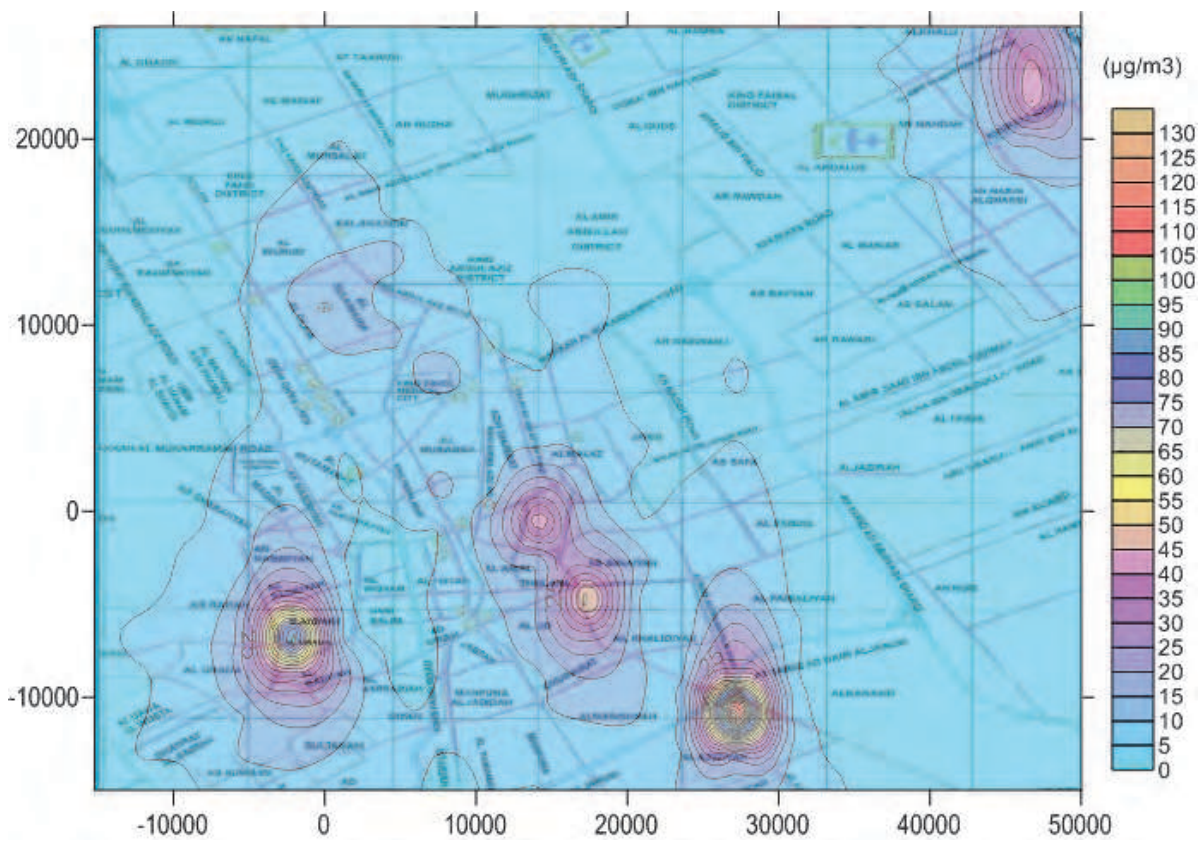
Fig. 4. (d) Distribution of \text{PM}_{10} for 12month period, the 24-hour maximum
