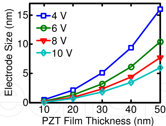
Fig. 9. Minimum electrode size for full-thickness domain inversions for various PZT thicknesses at different applied biases (Tayebi et al., 2010a).
