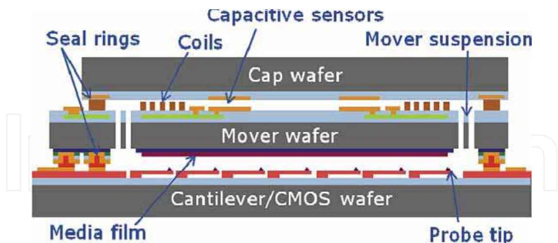
Fig. 3. Schematic of Intel SSP memory device architecture (Heck et al., 2010).
