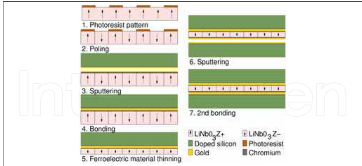
Fig. 15. Flowchart which summarizes the different steps of fabrication
