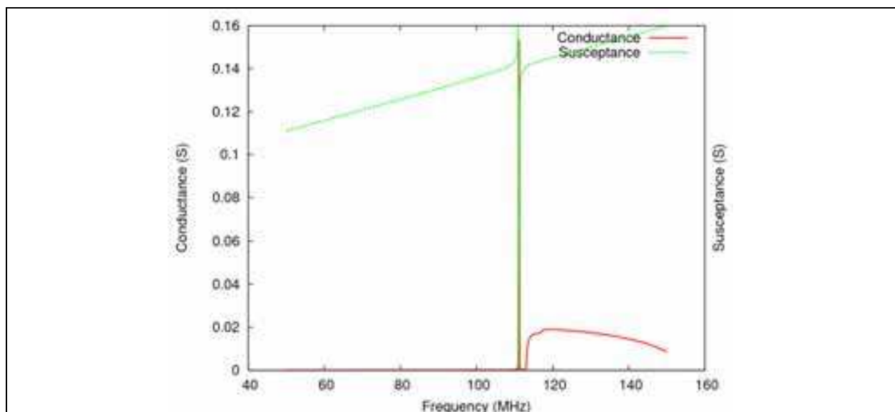
Fig. 14. Example of harmonic admittance computed for a Si/LiNbO 3 /Si transducer/waveguide, the period of the PPT (wavelength) is 50 μm, the niobate layer is 30 μm thick (the pole is the signature of a guided mode).
