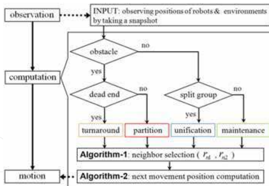
Fig. 5. Adaptive navigation algorithm flowchart
