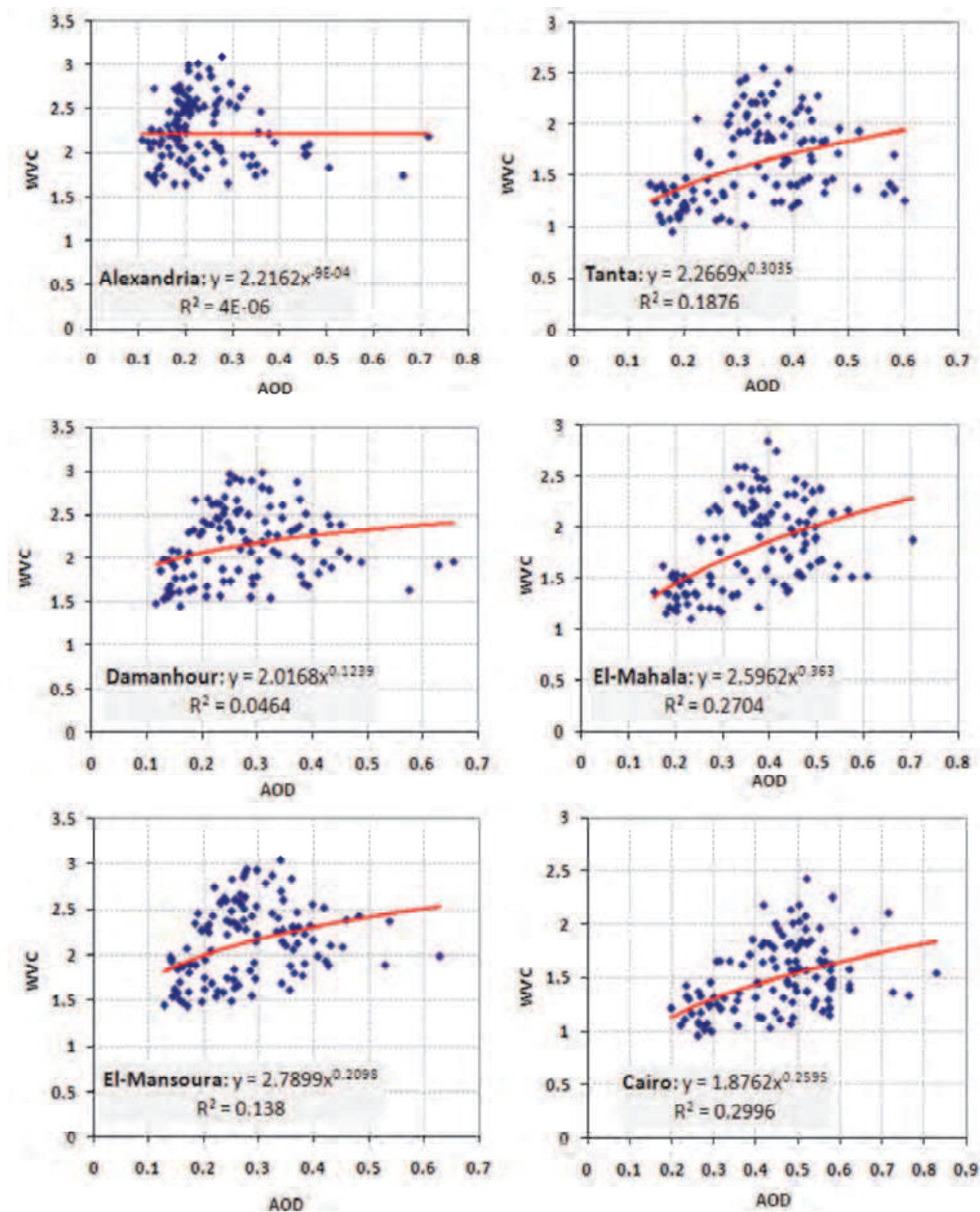
Fig. 6. Power correlation between MODIS AOD and MODIS water vapor (near infra-red, clear column) from February 2000 till May 2009 the six cities.
