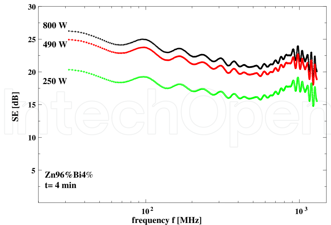
Fig. 13. The coefficient of shielding efficiency SE versus frequency f , for different powers released on the Zn96%Bi4% target in case of unipolar DC-M supply.
