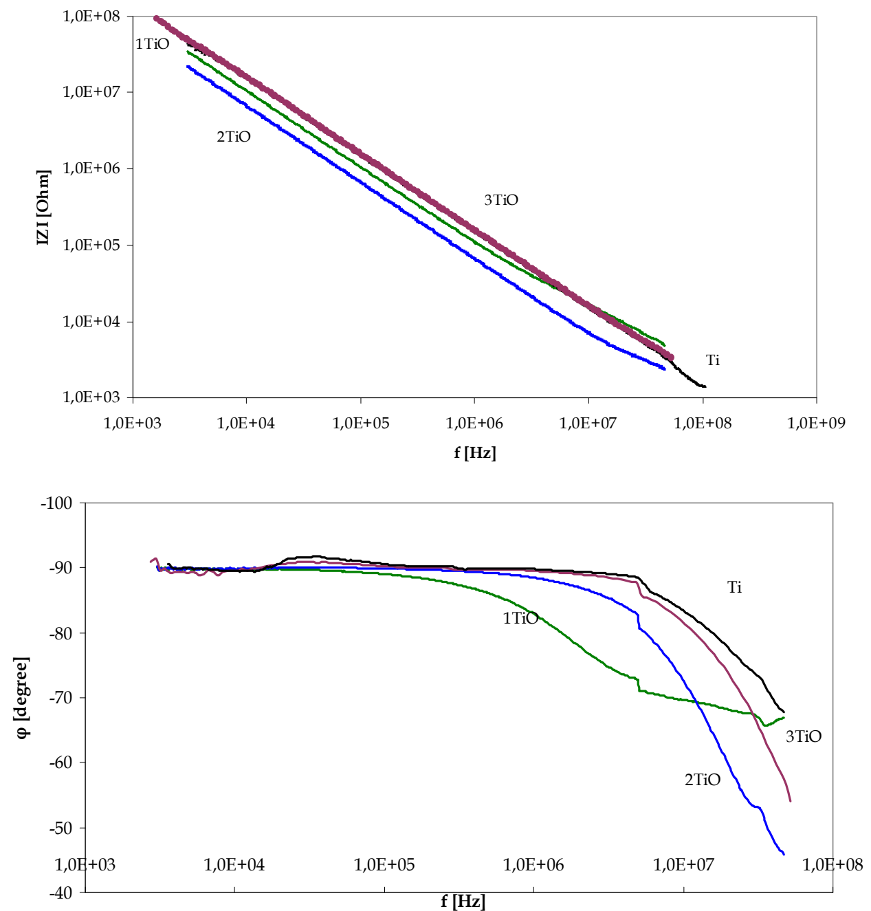
Fig. 16. The Bode diagram of examined composite structures.
