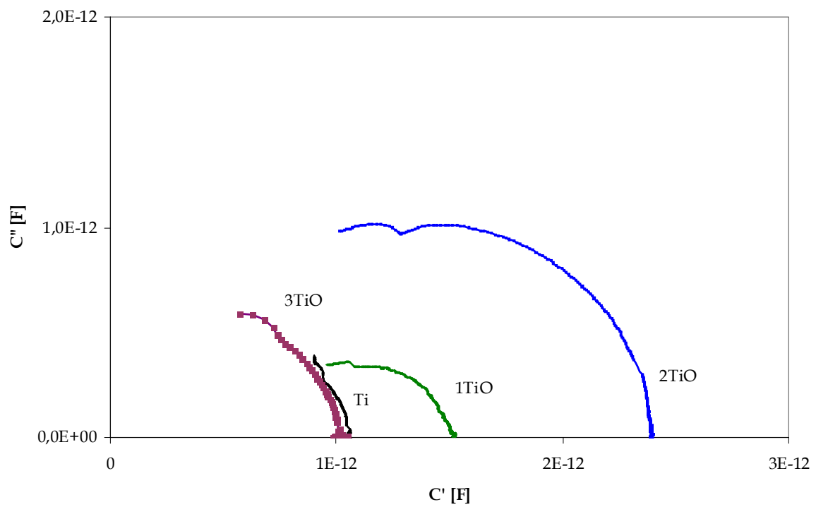
Fig. 19. The Cole-Cole diagram of the complex capacitance
