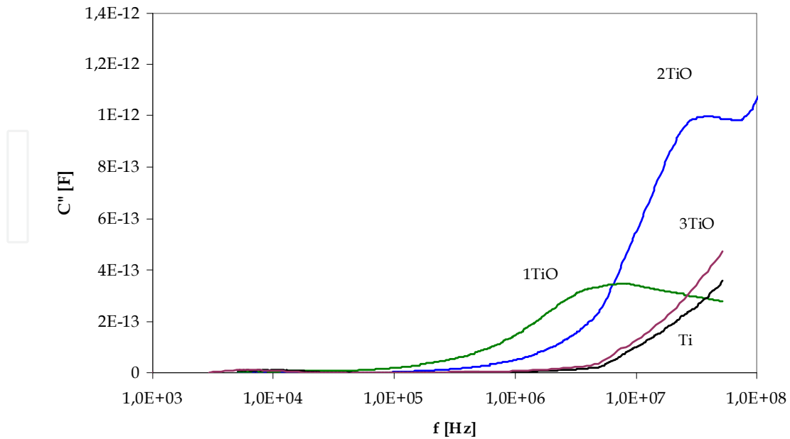
Fig. 18. Frequency spectrums of imaginary component of complex capacitance.
