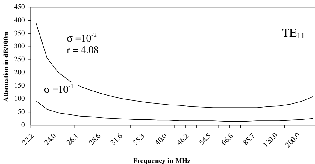
Fig. 1. Frequency and attenuation in a circular tunnel
