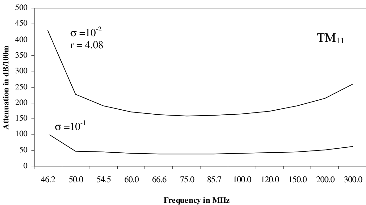
Fig. 3. Frequency and attenuation in a circular tunnel
