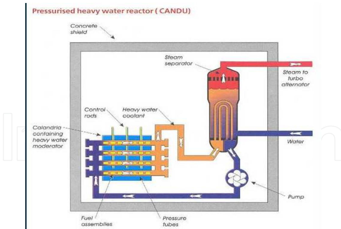
Figure 1.14 CANDU Reactor
