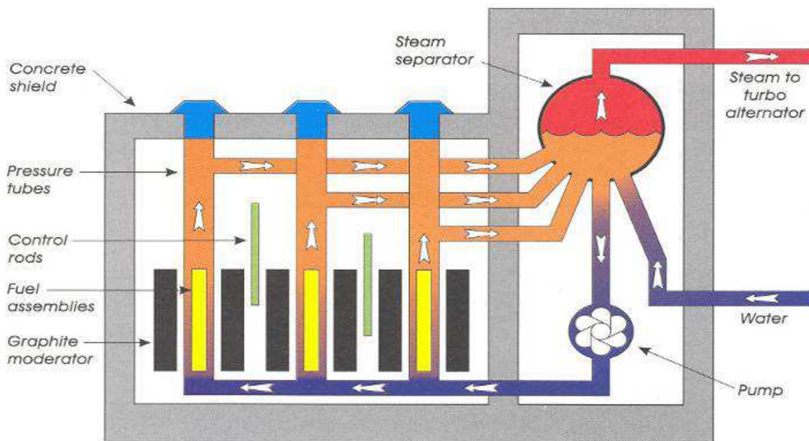
Figure 1.9 RBMK Reactors
