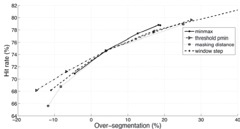
Fig. 5. Effects of different parameter values on segmentation results tested independently of each other. Parameter ranges are n_{mm} = 20-100 ms, t_d = 5-45 ms, ws = 1-3 ms and p_{min} = 0.02-0.1 . Adjustment of the values changes the trade-off balance between hit-rate and over-segmentation, but the slope decreases as the value of over-segmentation increases.
